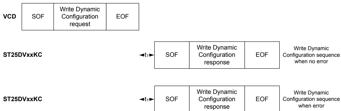
Figure 63. Write Dynamic Configuration frame exchange between VCD and ST25DVxxKC
