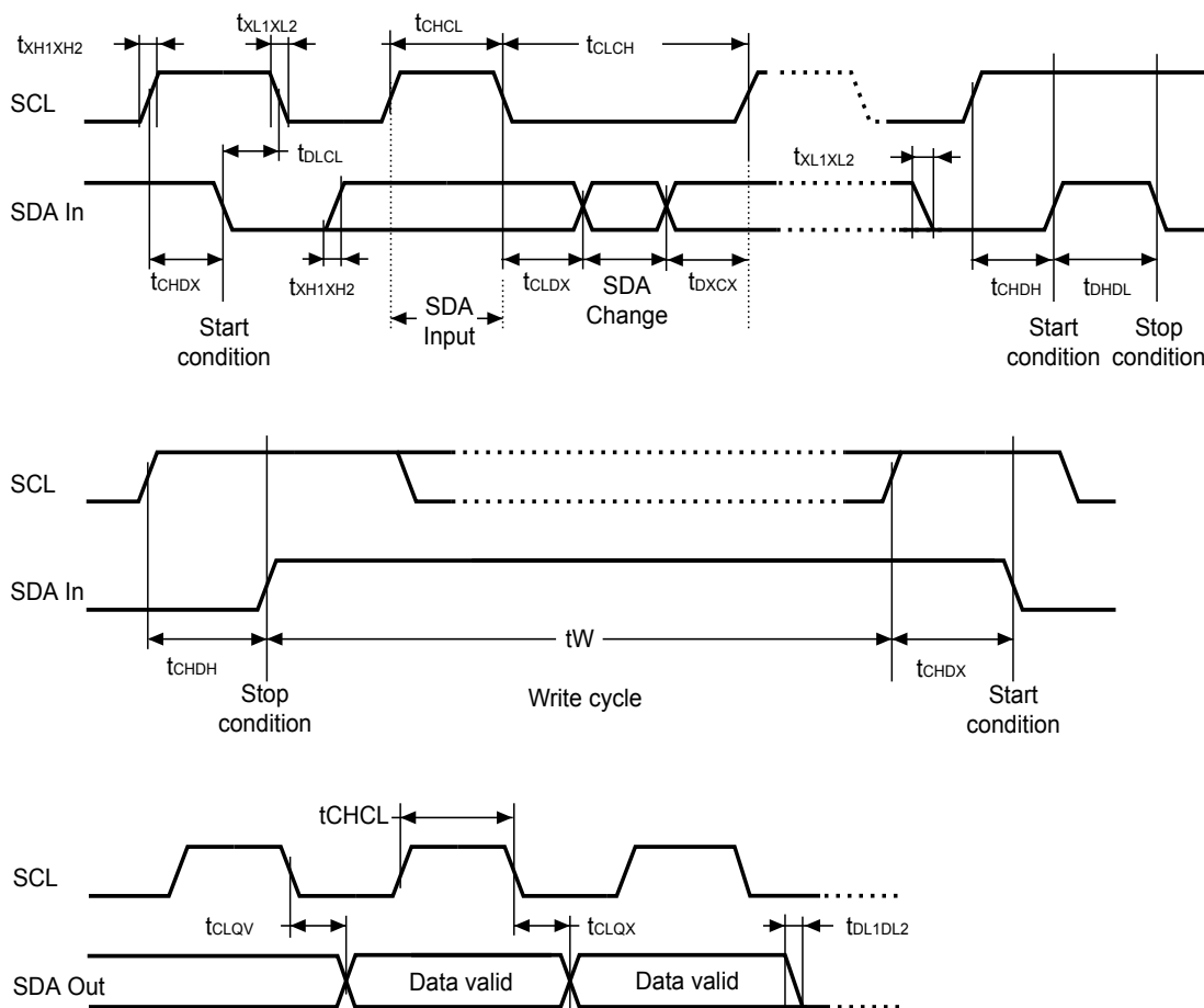
Figure 80. I 2 C AC waveforms
