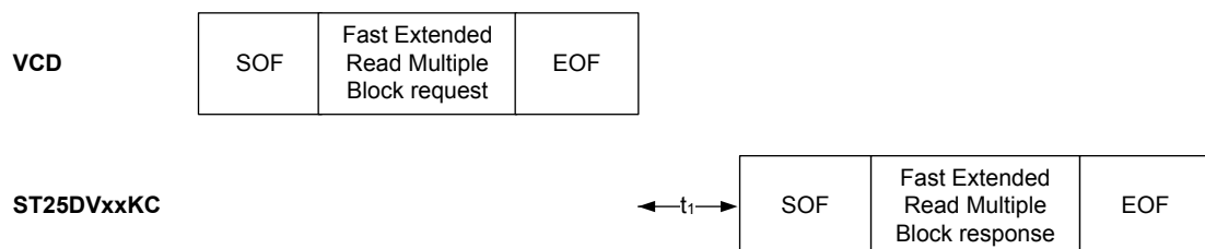
Figure 74. Fast Extended Read Multiple Block frame exchange between VCD and ST25DVxxKC
