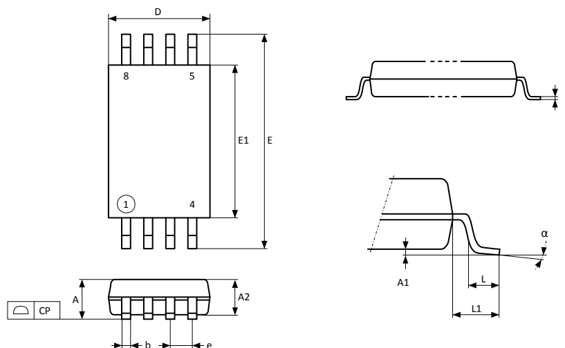
Figure 85. TSSOP8 – Outline
