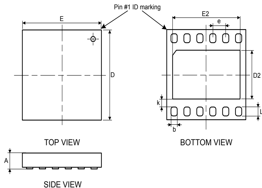
Figure 88. UFDFPN12 - Outline
