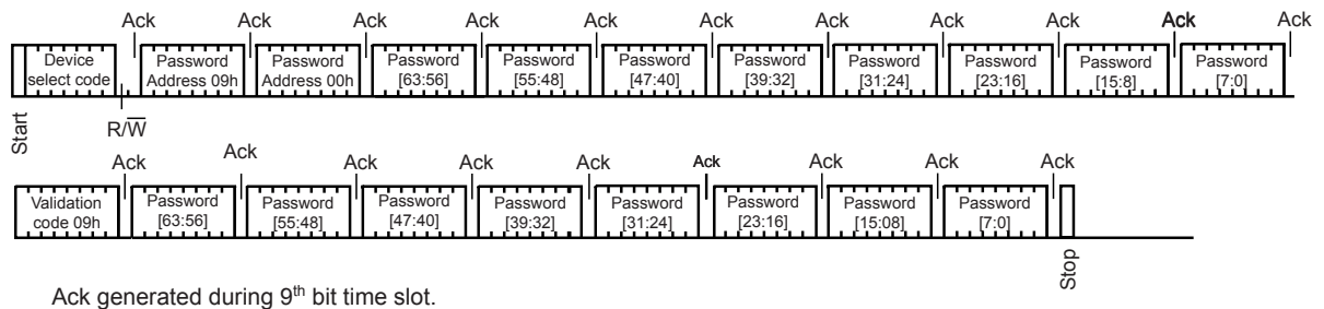
Figure 35. I 2 C Present Password Sequence
