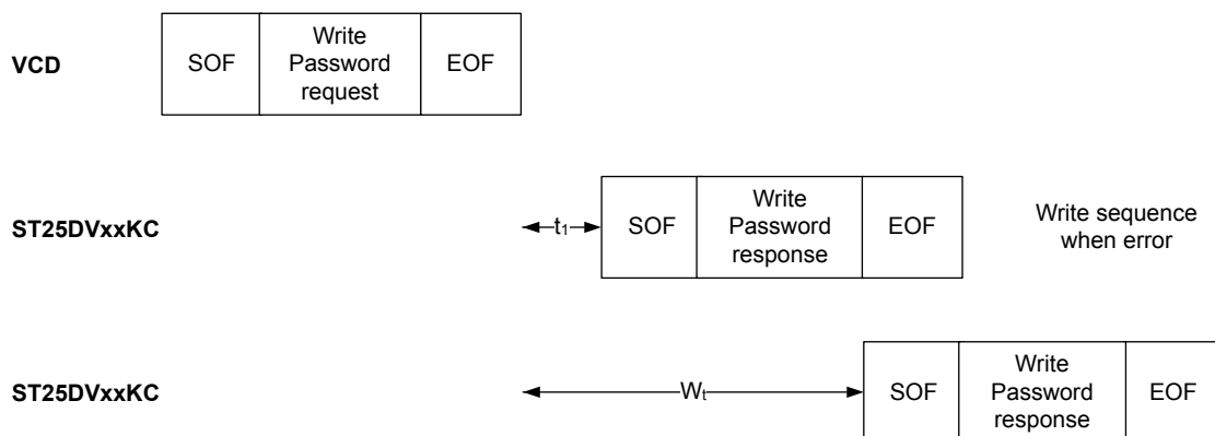
Figure 69. Write Password frame exchange between VCD and ST25DVxxKC
