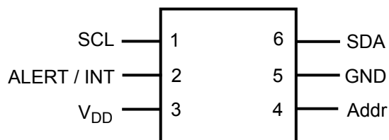
Figure 1. Pin configuration
