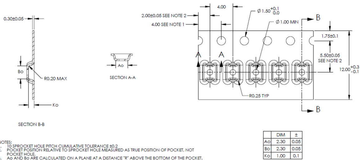
Figure 12. Carrier tape information for UDFN-6L package
