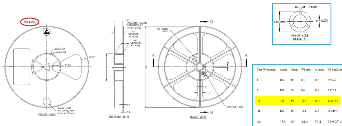
Figure 14. Reel information
