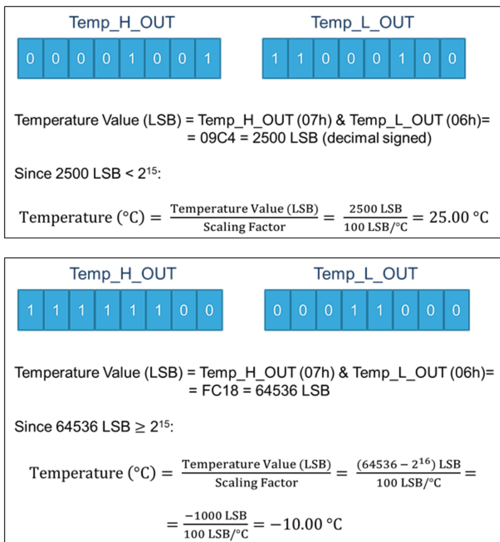
Figure 7. Temperature readings
