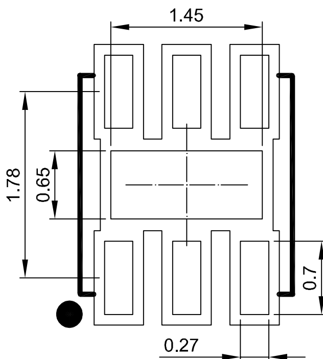
Figure 10. Land pattern
