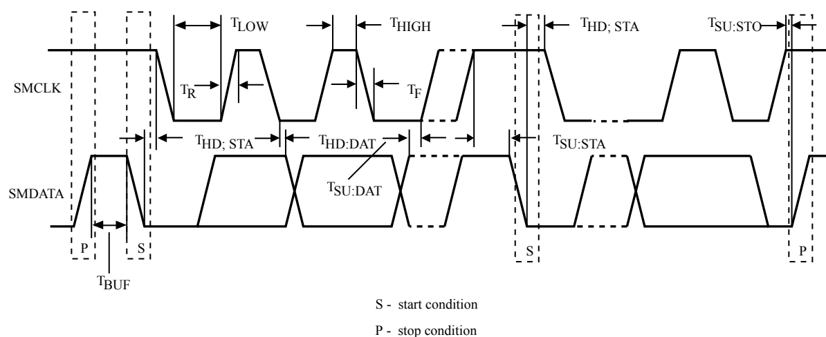
Figure 3. SMBus timing diagram
