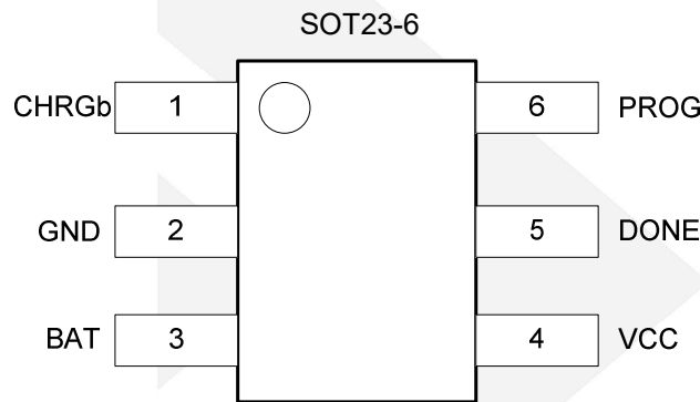
Figure 2 Pin Assignment
