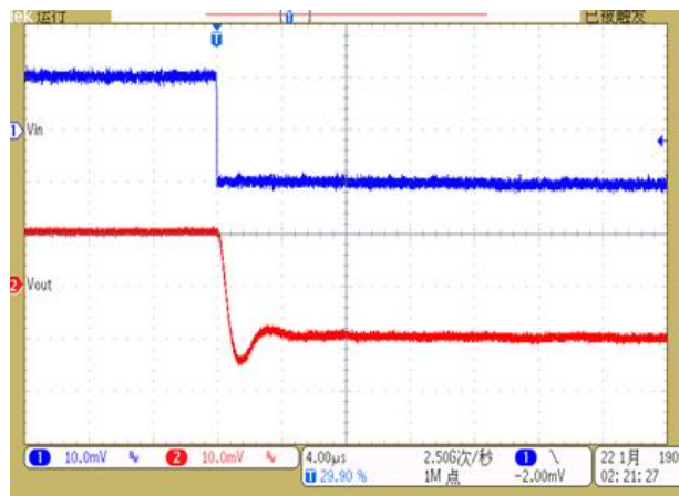
Figure 7. Small-signal response
