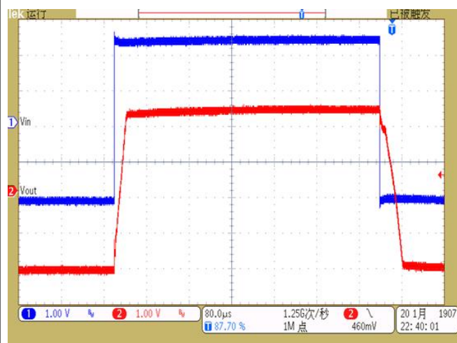
Figure 6. Small-signal response
