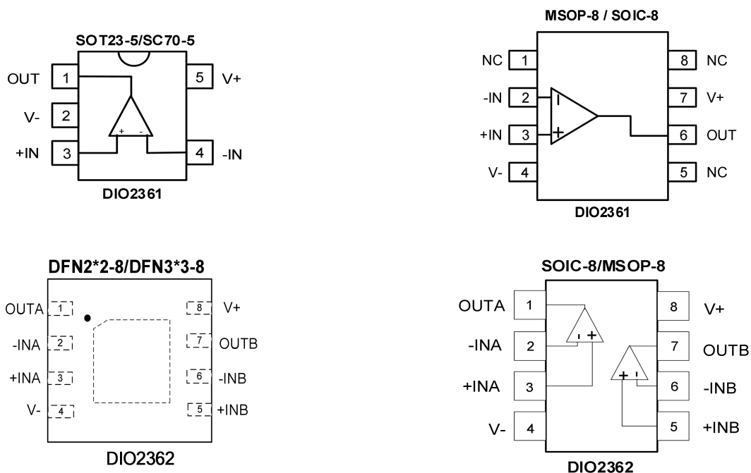
Figure 1. Top view
