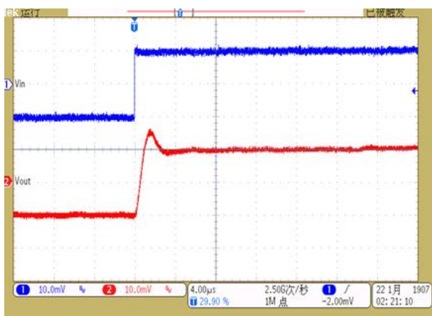
Figure 6. Small-signal response
