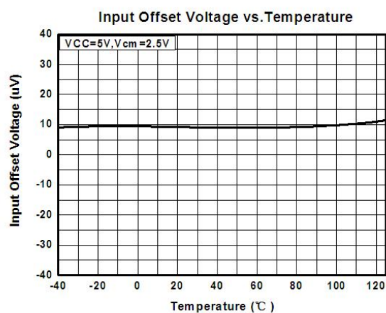
Figure 5. V_{OS} vs. Temperature
