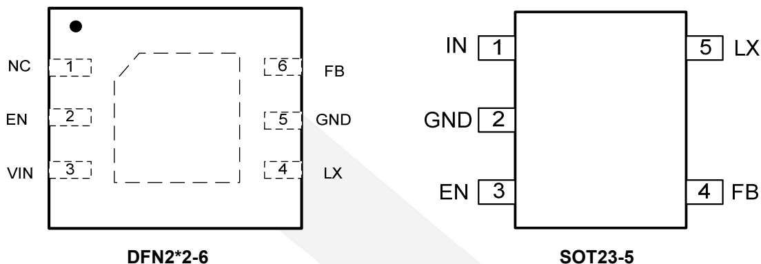
Figure 1 Pin Assignment (Top View)
