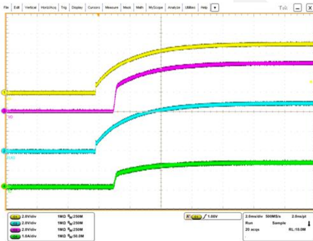
( V_{IN} = 5\text{ V} , V_{EN} = V_{IN} , R_{OUT} = 3.9\ \Omega , V_{IN} \rightarrow 0\text{ V} ) Figure 16. UVLO
