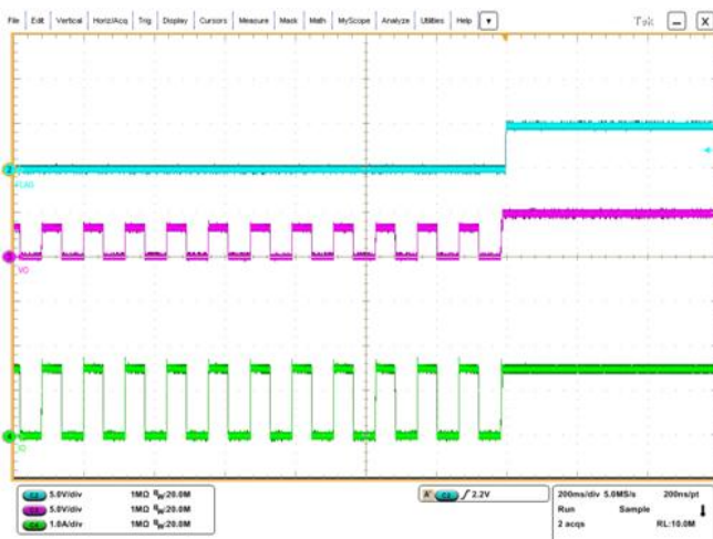
( V_{IN} = 5\text{ V} , V_{EN} = V_{IN} , R_{OUT} = 1.8 \rightarrow 3.3\ \Omega ) Figure 19. Overload to heavy load recovery
