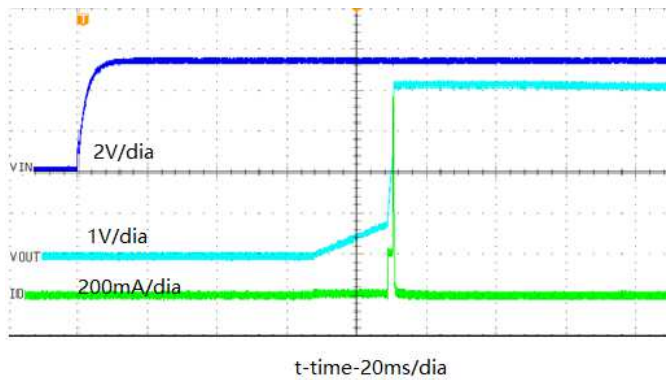
Figure 6. AC Charging
