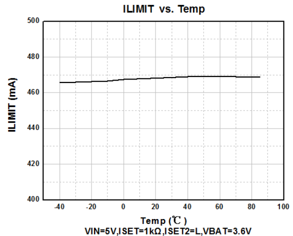
Figure 9. ILIMIT vs. Temp
