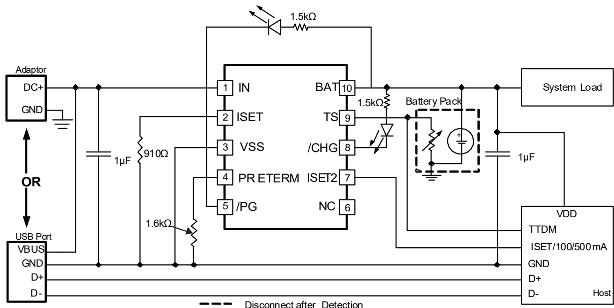
Figure 3. Typical Applications for DIO5090C
