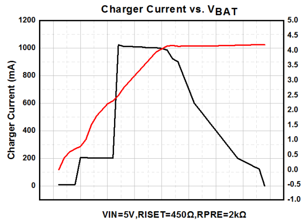
Figure 7. Charger Current vs. V_{BAT}
