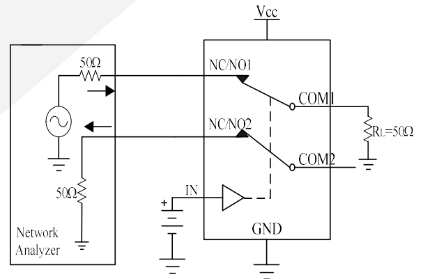
Figure 6 Channel-to-channel crosstalk
