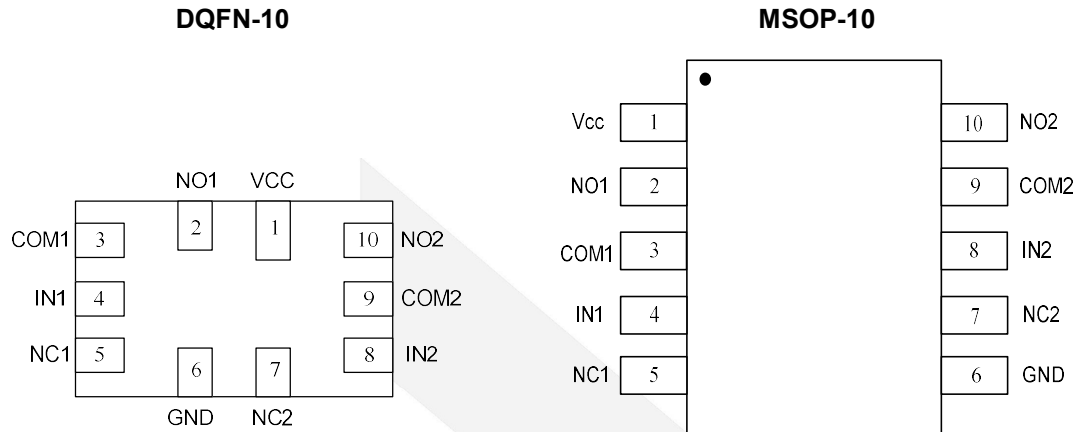
Figure 1 Top View
