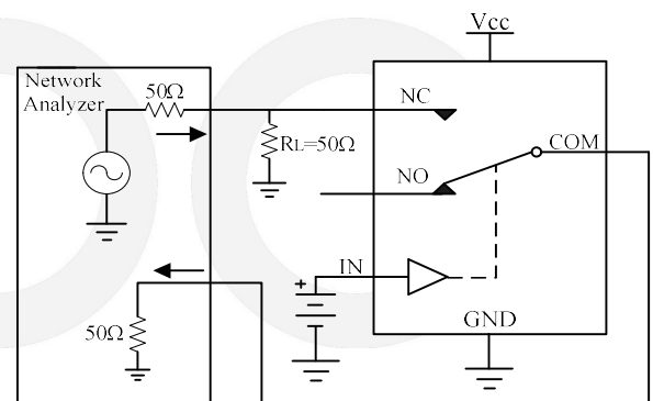
Figure 7 Off-isolation
