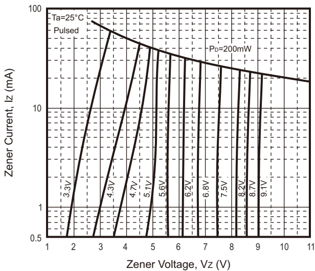
Fig.1 - Zener Characteristics ( V_z up to 9.1V)
