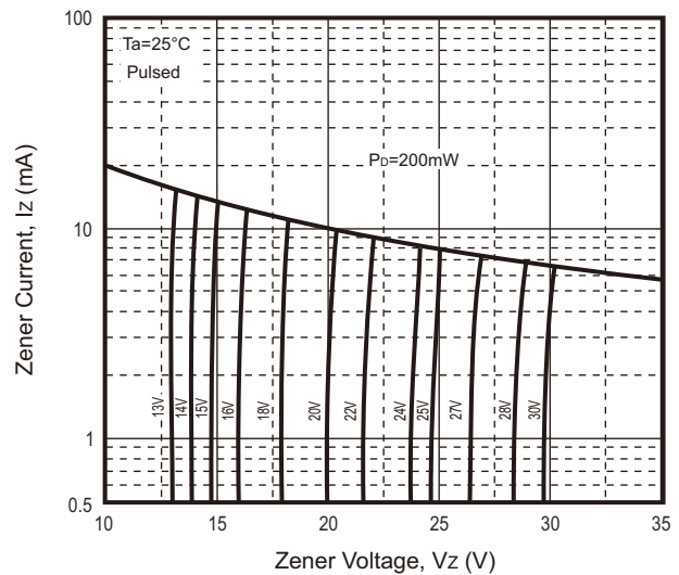
Fig.2 - Zener Characteristics (13V to 30V)
