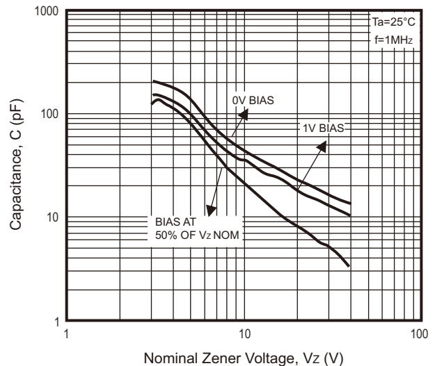
Fig.4 - Typical Capacitance
