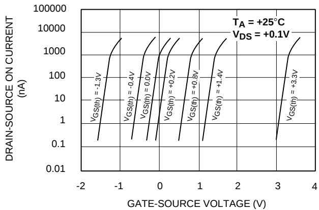
SUBTHRESHOLD FORWARD TRANSFER CHARACTERISTICS
