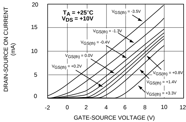
FORWARD TRANSFER CHARACTERISTICS
