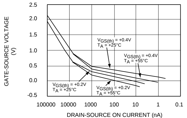
SUBTHRESHOLD CHARACTERISTICS
