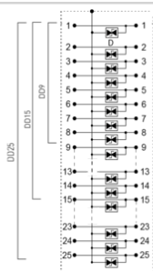
D: Clamping diode
