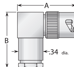
Figure 4 (Military clamp)
