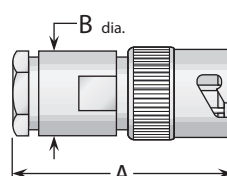
Figure 3 (Military clamp)
