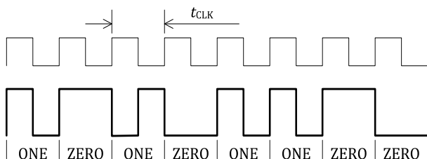
Figure 5. Example of a differential bi-phase encoding scheme
