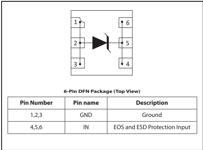
Figure 6 - Pin Configuration and Description
