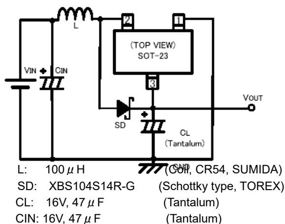
●A type circuit
