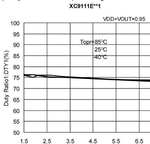
(14) Duty Ratio 1 vs. Output Voltage
