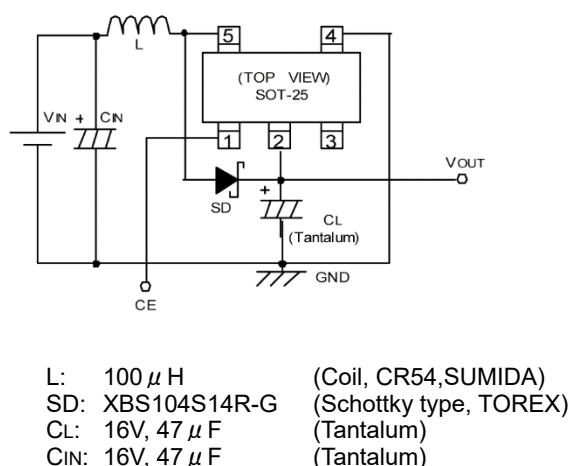
●C type circuit
