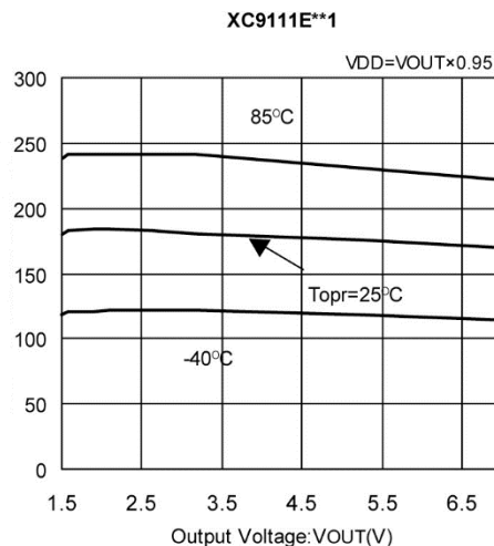
(15) Duty Ratio 2 vs. Output Voltage
