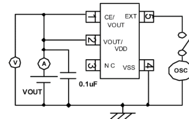
Circuit ⑦
