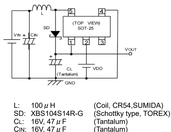
●E type circuit
