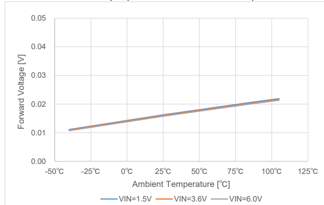
(8-2-1) Forward Voltage vs Ambient Temperature
