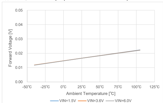
(8-2-2) Forward Voltage vs Ambient Temperature
