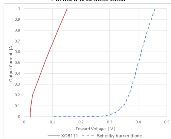
Forward characteristics
