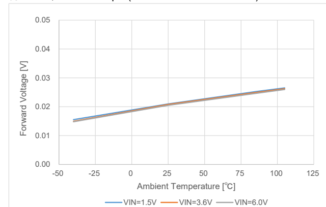
(6-2-2) Forward Voltage vs Ambient Temperature
