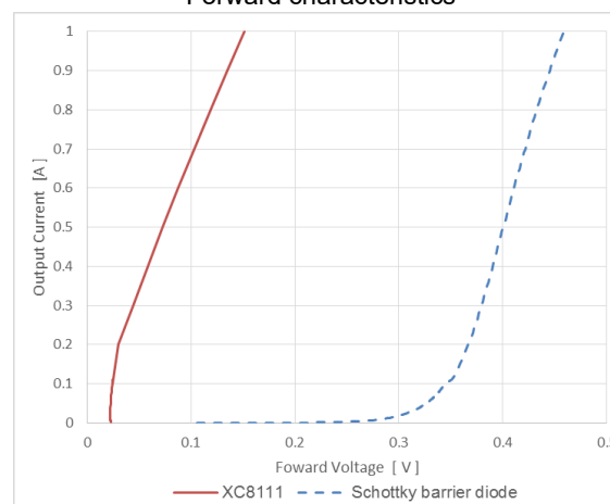
Forward characteristics
