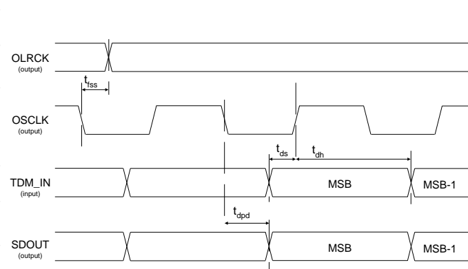
Figure 4. TDM Master Mode Timing
