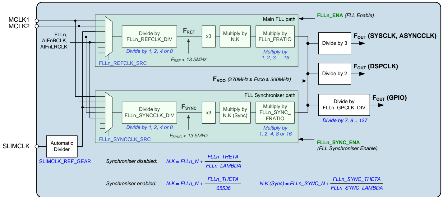
Figure 76 FLL Configuration
