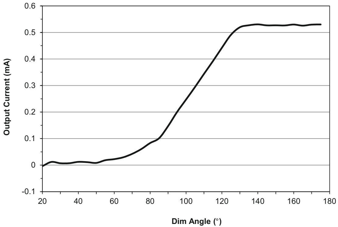
Figure 9. Typical Output Current vs. Dim Angle
