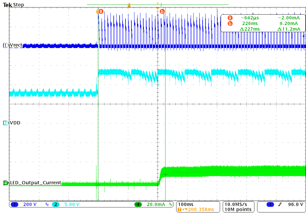
Figure 20. ILED at Minimum Dim Angle, Turn-on Waveforms
