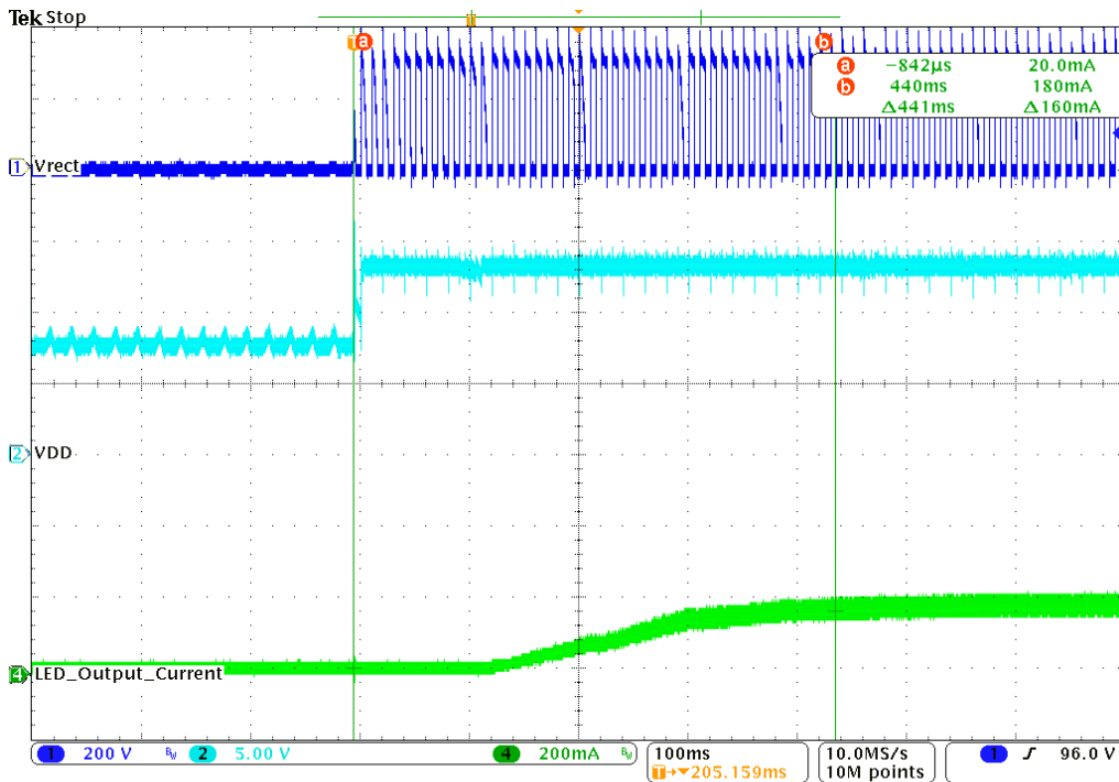
Figure 19. ILED at Medium Dim Angle, Turn-on Waveforms
