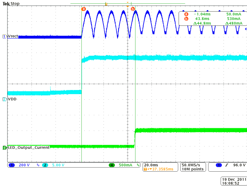
Figure 14. No-dimmer Mode, Startup 230VAC
