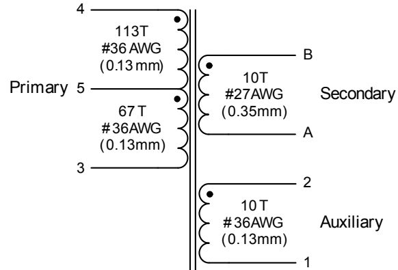
Figure 8. Flyback Transformer Schematic
