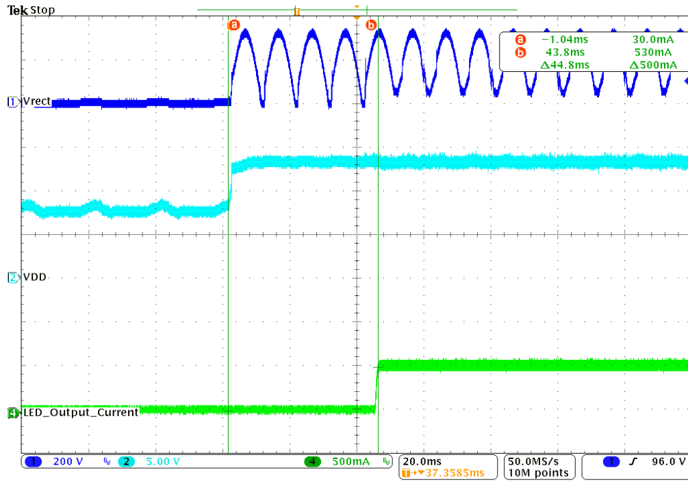
Figure 18. ILED at Maximum Dim Angle, Turn-on Waveforms
