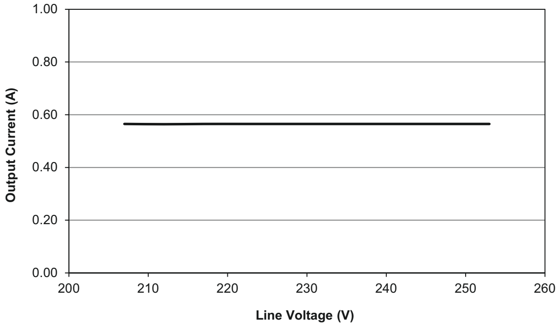
Figure 11. Output Current vs. Line Voltage
