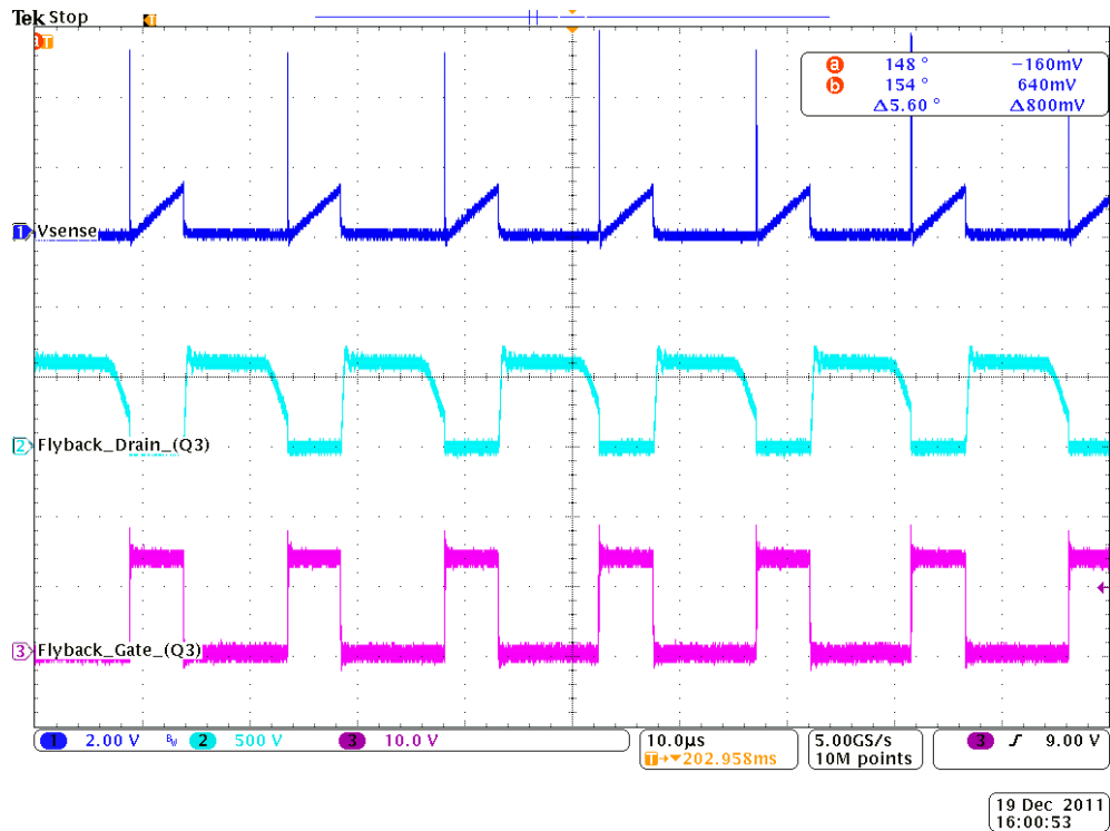
Figure 17. Flyback FET, Q3, Waveform
