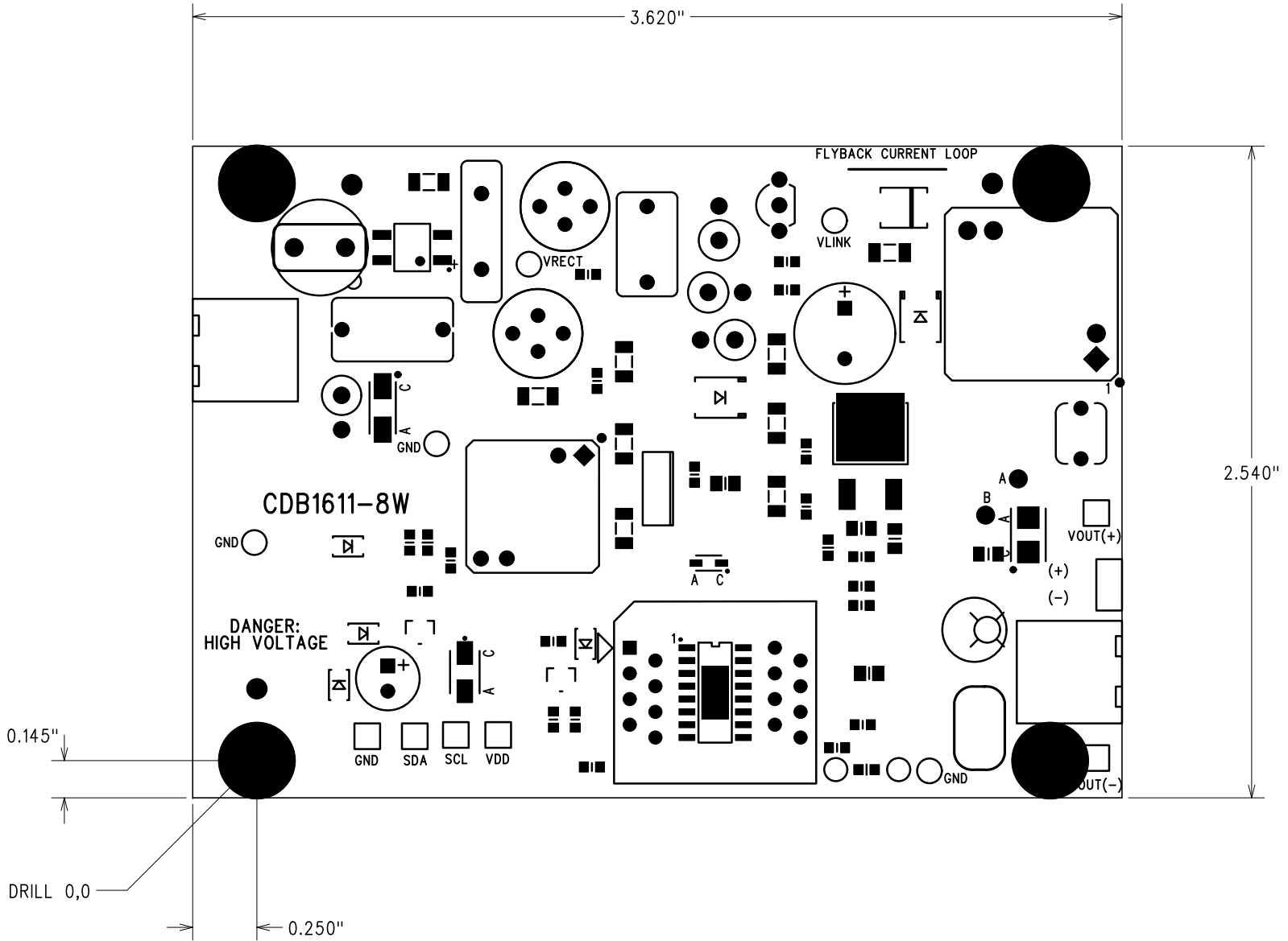
Figure 3. PCB Dimensions
