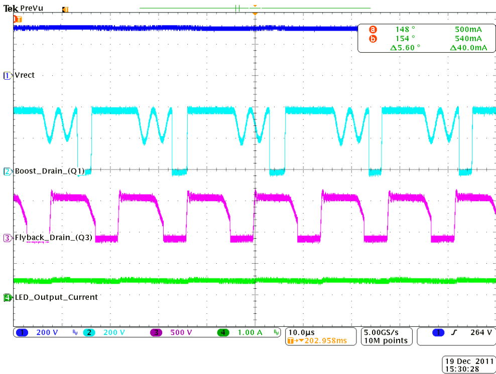
Figure 15. No-dimmer Mode, Steady-state, 230VAC
