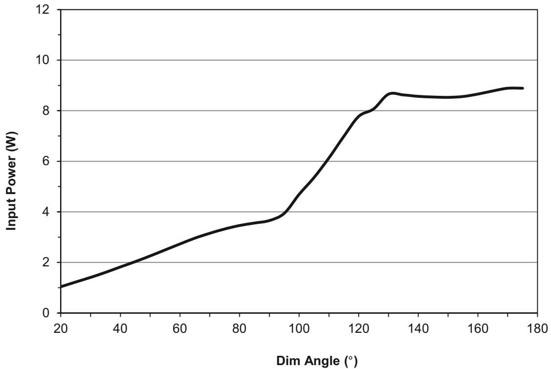
Figure 10. Typical Input Power vs. Dim Angle
