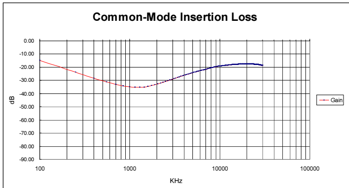
Typical Common-mode Loss for FM30R100P
