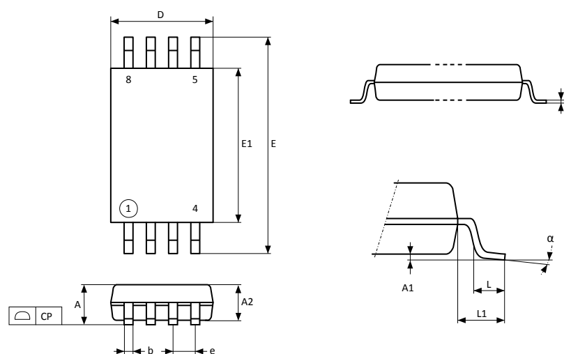
Figure 80. TSSOP8 – Outline
