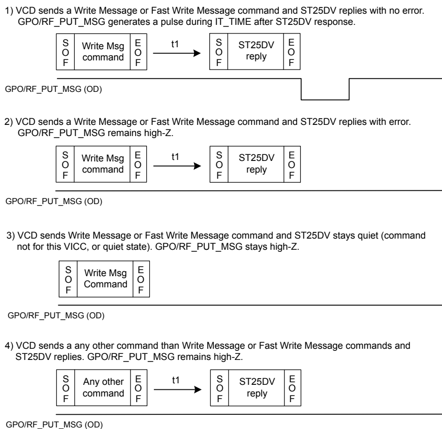
Figure 16. RF_PUT_MSG chronogram
