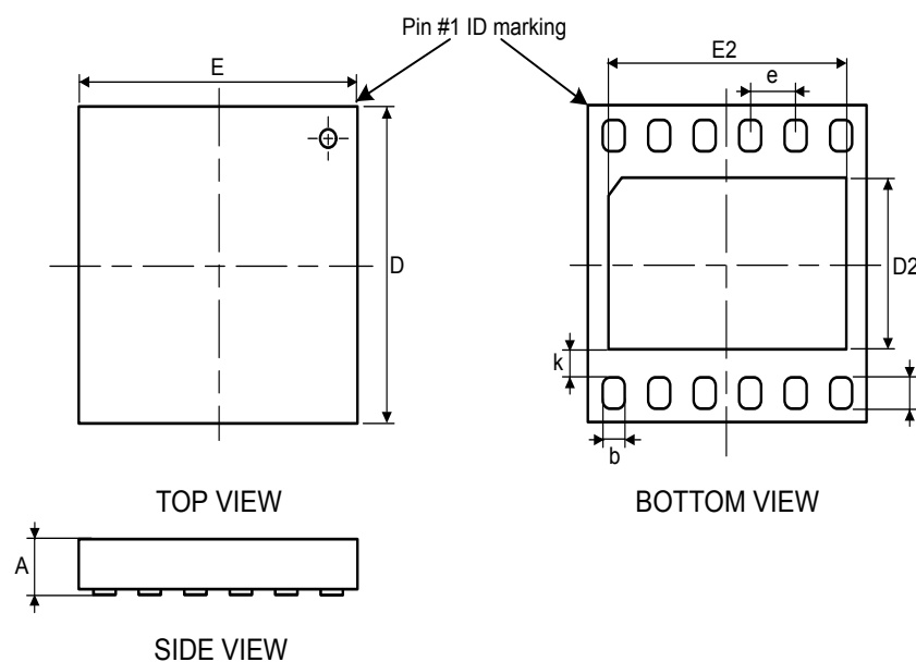
Figure 83. UFDFPN12 - Outline
