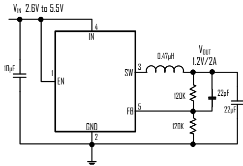
1.2V/2A 3MHz Step-Down Converter
