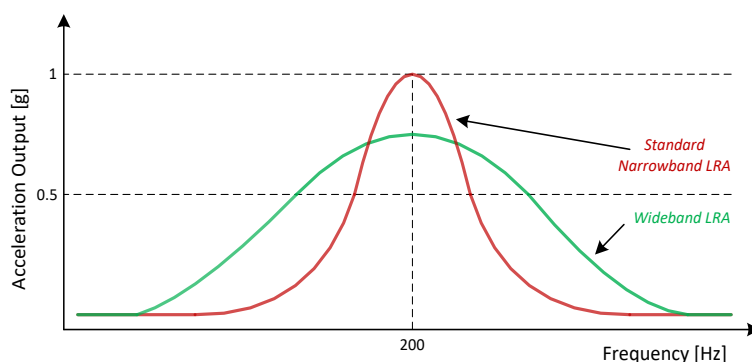
Figure 6: Narrowband and Wideband LRA Response across Frequency
