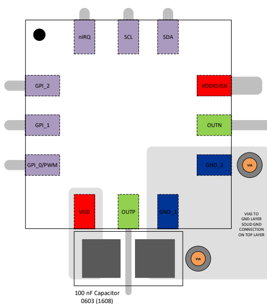
Figure 44: QFN Example PCB Layout
