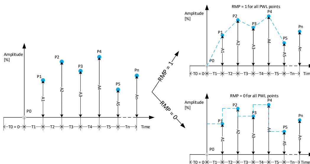
Figure 27: Snippet Example
