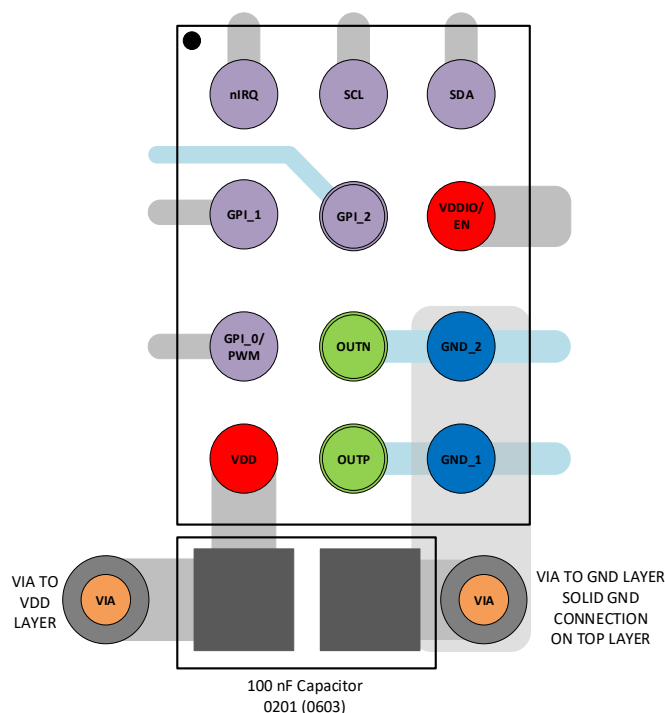
Figure 43: WLCSP Example PCB Layout
