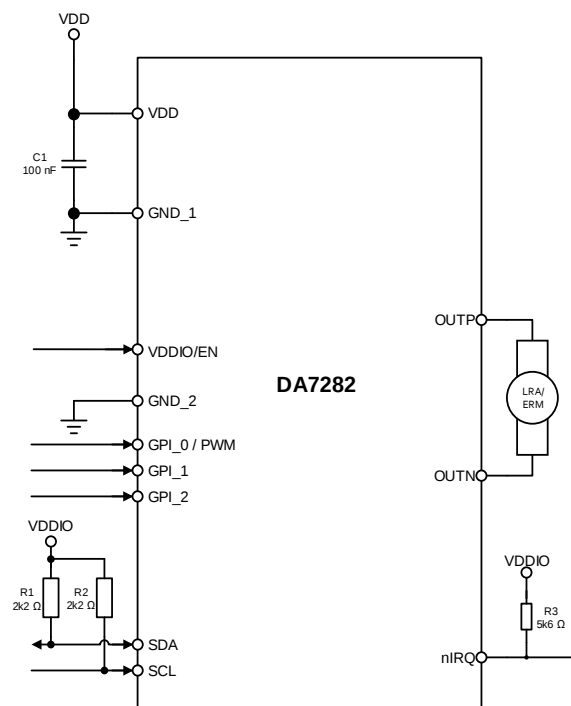
Figure 42: External Components Diagram
