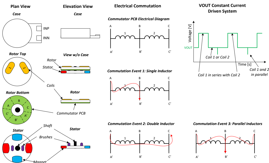
Figure 23: Coin ERM Physical and Electrical Summary
