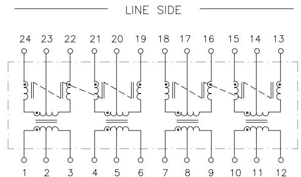
Circuit B
