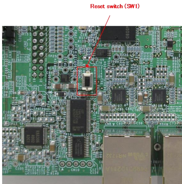
Figure 5-3 Reset switch
