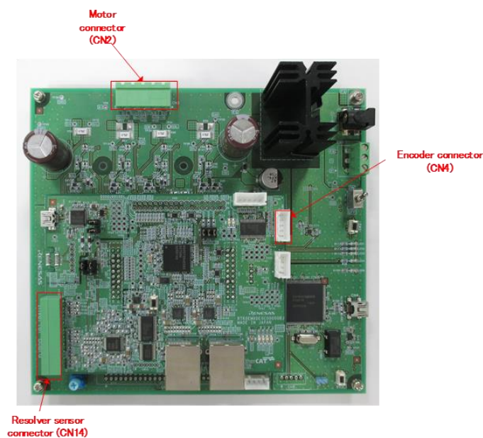
Figure 4-3 Motor and board Connection
