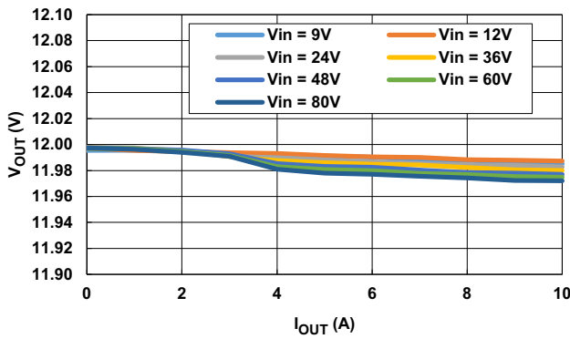
Figure 16. Load Regulation, CCM
