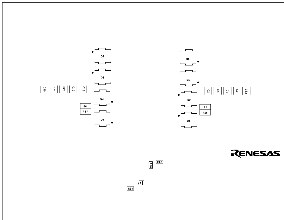
Figure 13. Silkscreen Bottom
