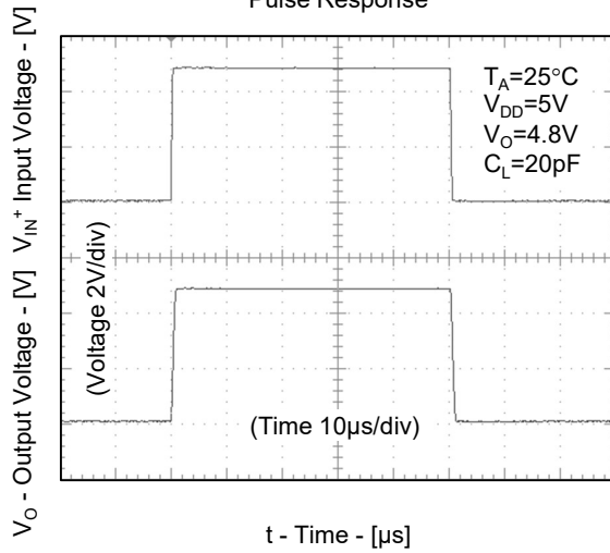
Pulse Response
