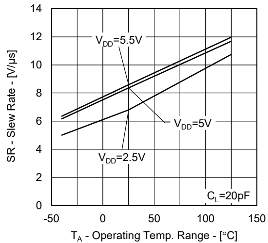
SR vs. T_A (Output Fall Time)
