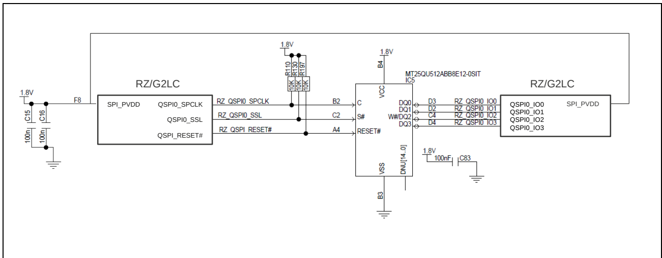
Figure 2.1 Block Diagram of QSPI I/F
