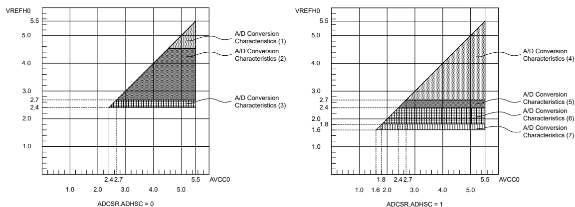
Figure 2.37 AVCC to VREFH0 voltage range
