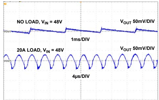
FIGURE 11. OUTPUT RIPPLE, MODE = DEM
