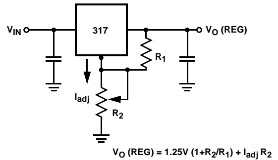
FIGURE 13. VOLTAGE REGULATOR
