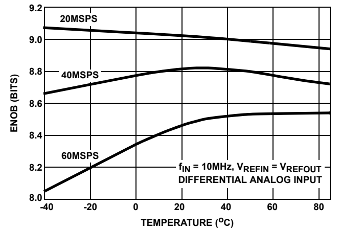
FIGURE 9. EFFECTIVE NUMBER OF BITS (ENOB) vs TEMPERATURE
