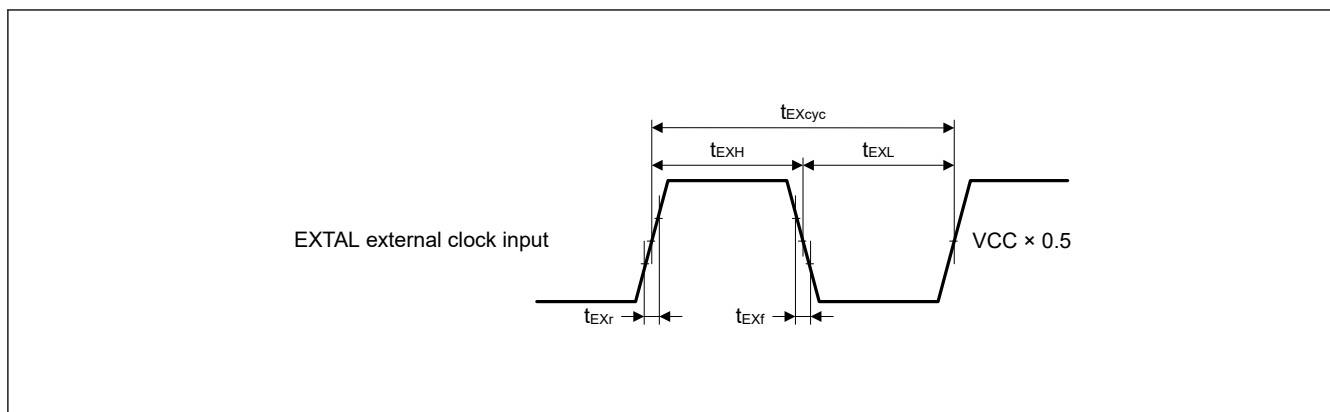
Figure 2.15 EXTAL external clock input timing
