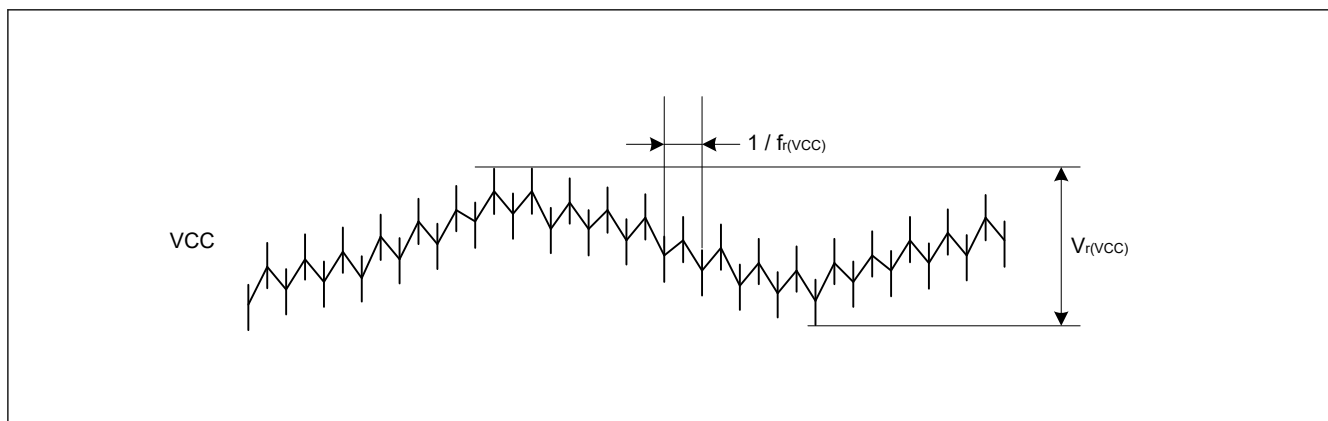
Figure 2.13 Ripple waveform
