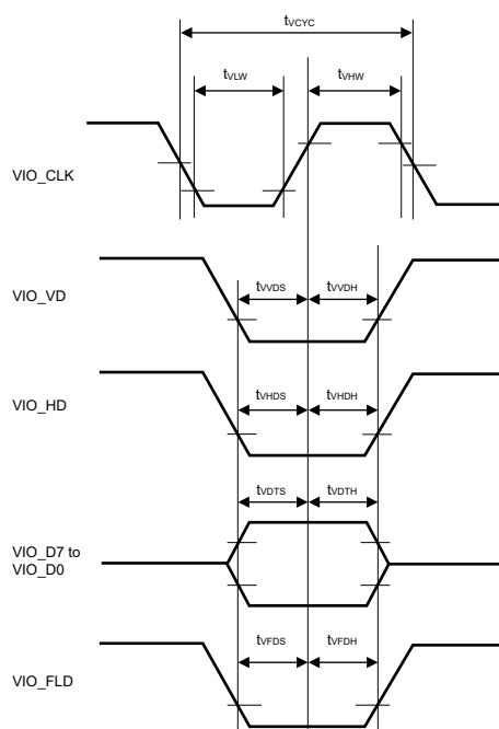
Figure 2.71 Capture Engine Unit Module Signal Timing of data capturing on the rising edge of VIO_CLK
