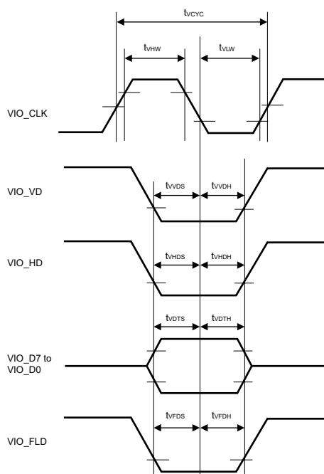
Figure 2.72 Capture Engine Unit Module Signal Timing of data capturing on the falling edge of VIO_CLK
