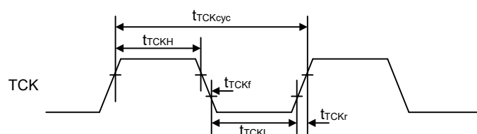
Figure 2.86 Boundary scan TCK timing
