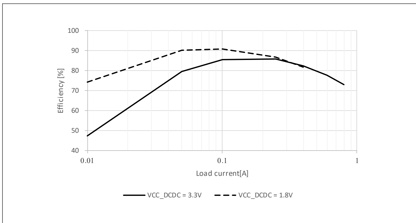
Figure 2.10 Typical DCDC efficiency (%) vs load current (A) in High-speed mode , T_j = 105^\circ\text{C}
