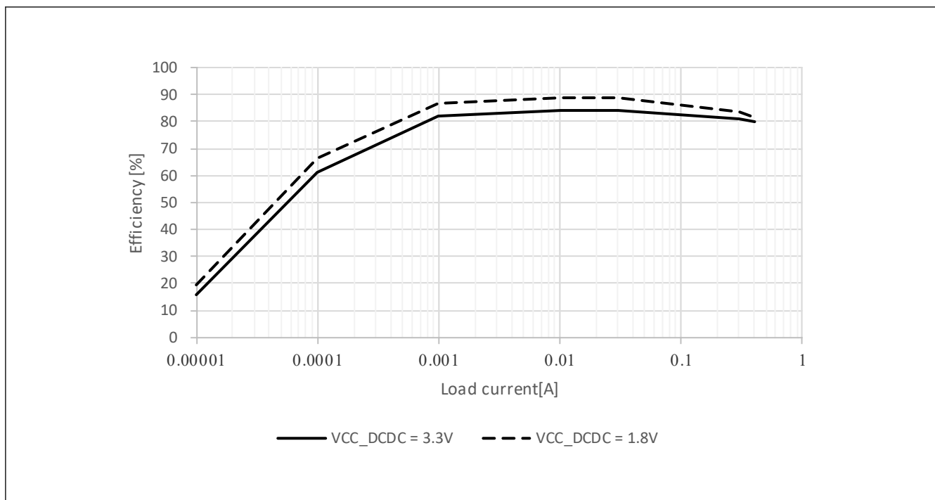
Figure 2.11 Typical DCDC efficiency (%) vs load current (A) in Low-speed mode and Software Standby mode, T_j = 25^\circ\text{C}
