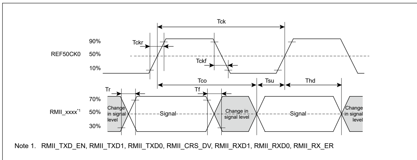
Figure 2.61 REF50CK0 and RMII signal timing
