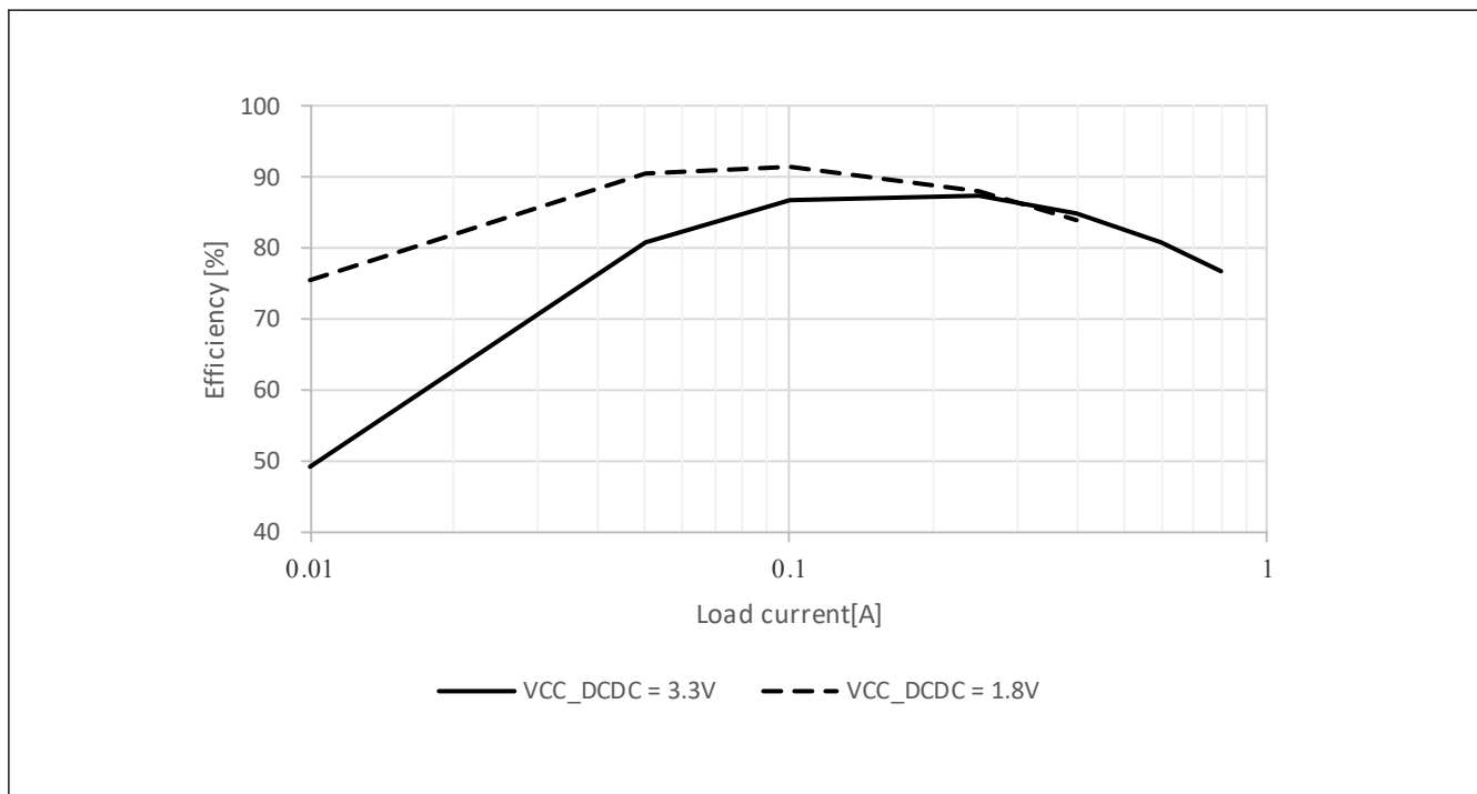
Figure 2.9 Typical DCDC efficiency (%) vs load current (A) in High-speed mode , T_j = 25^\circ\text{C}
