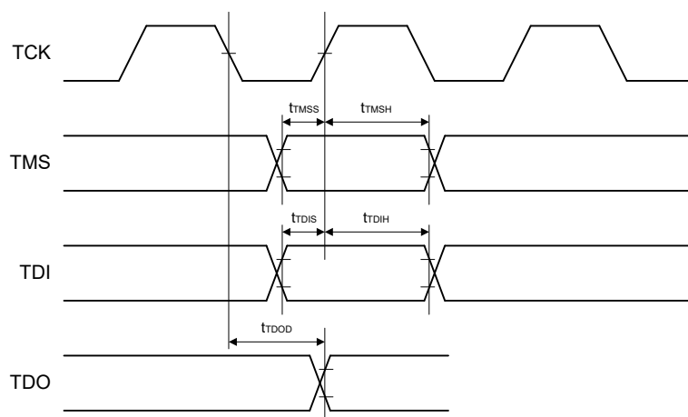
Figure 2.87 Boundary scan input/output timing (1)
