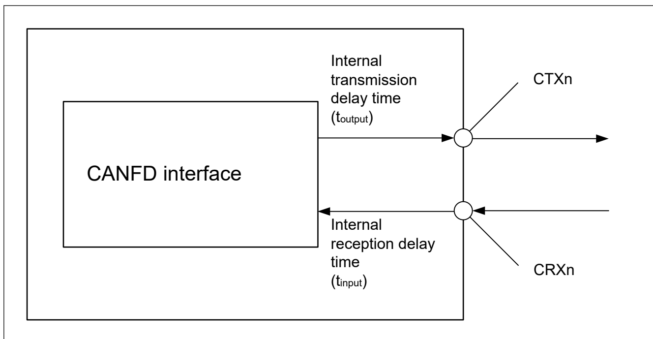
Figure 2.73 CANFD interface condition
