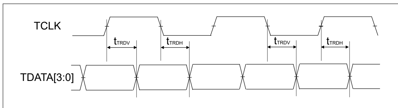
Figure 2.95 ETM output timing
