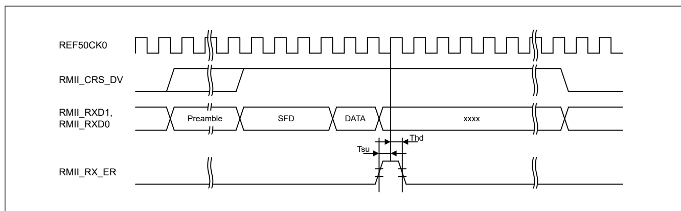
Figure 2.64 RMII reception timing when an error occurs
