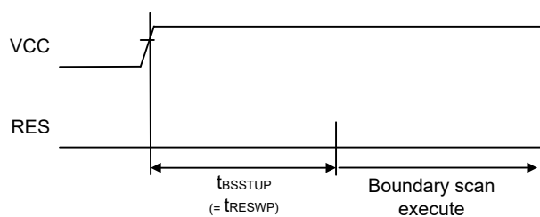
Figure 2.89 Boundary scan circuit startup timing
