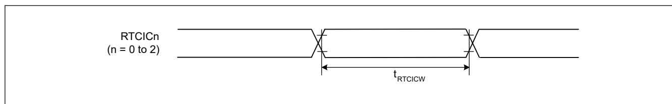
Figure 2.28 RTCICn input timing
