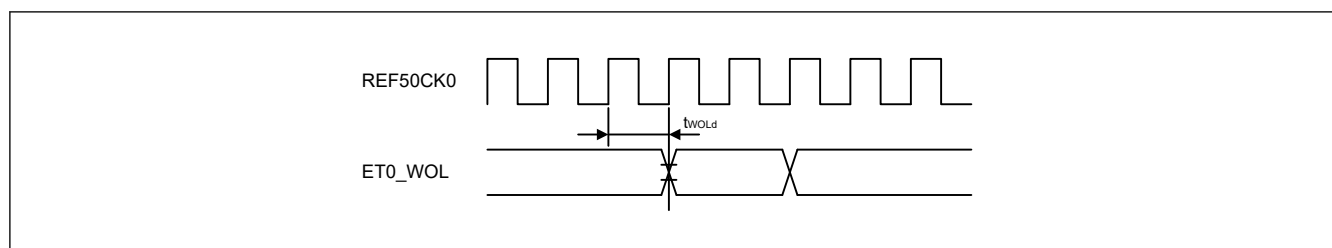
Figure 2.65 WOL output timing for RMII
