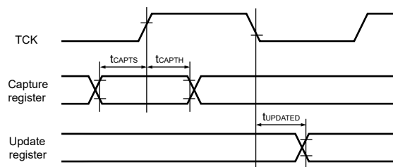
Figure 2.88 Boundary scan input/output timing (2)
