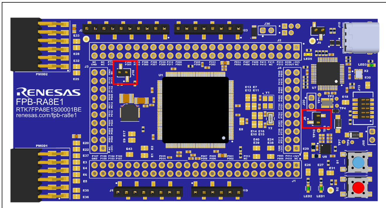
Figure 17. Boot Mode Jumpers (J6 and J16)
