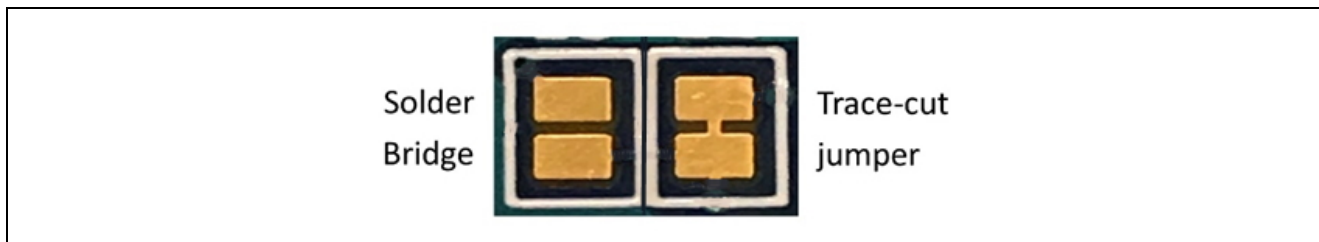
Figure 5. Copper Jumpers
