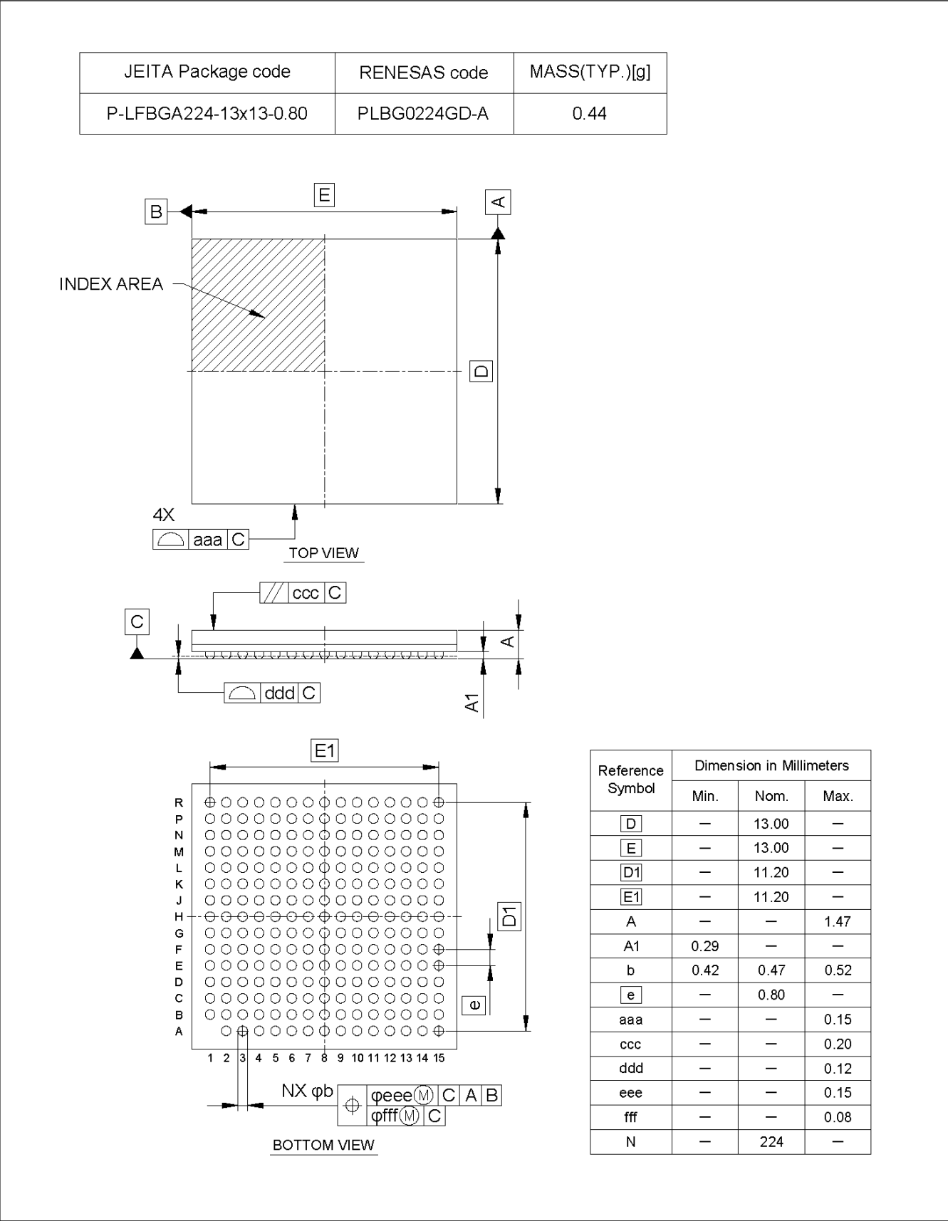
Figure 2.1 BGA 224-pin
