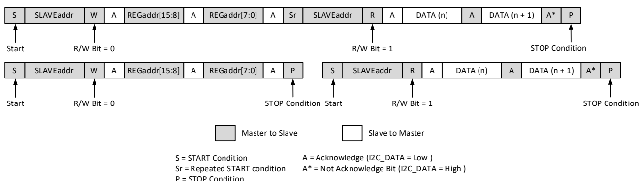
Figure 15. I²C Page Read Mode
