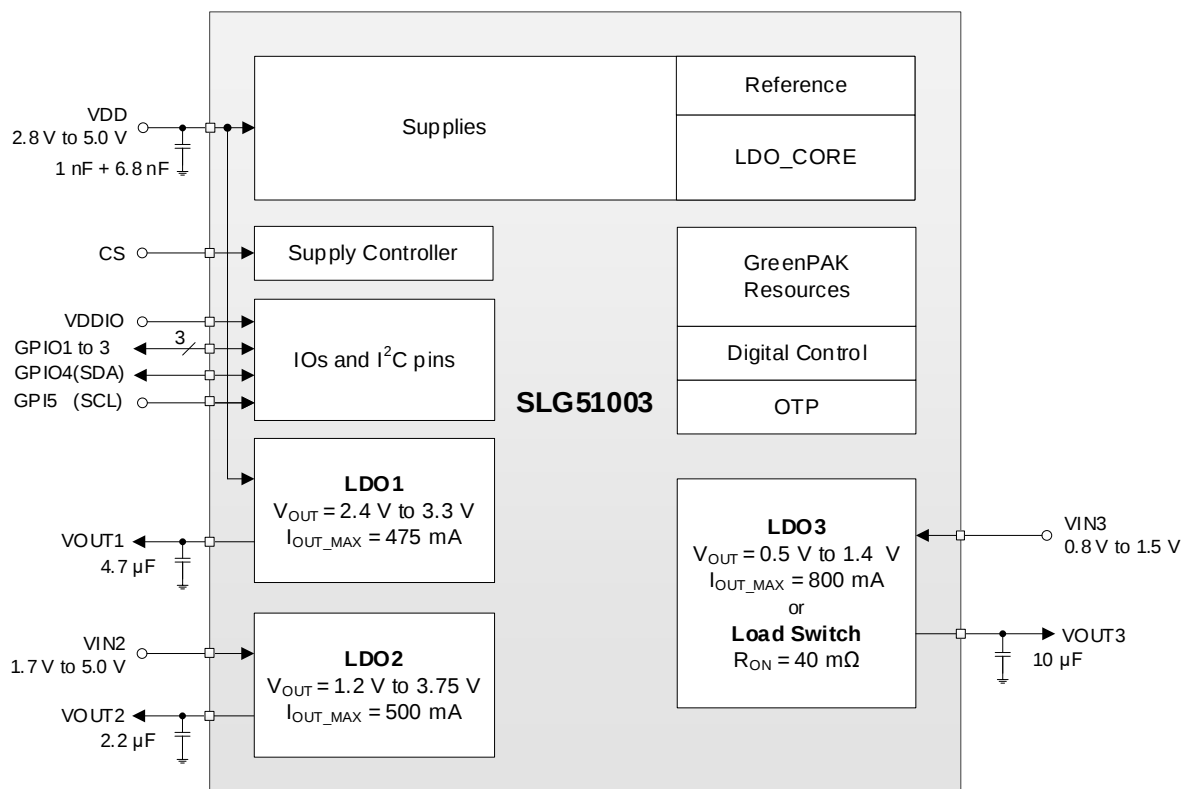
Figure 1. Block Diagram
