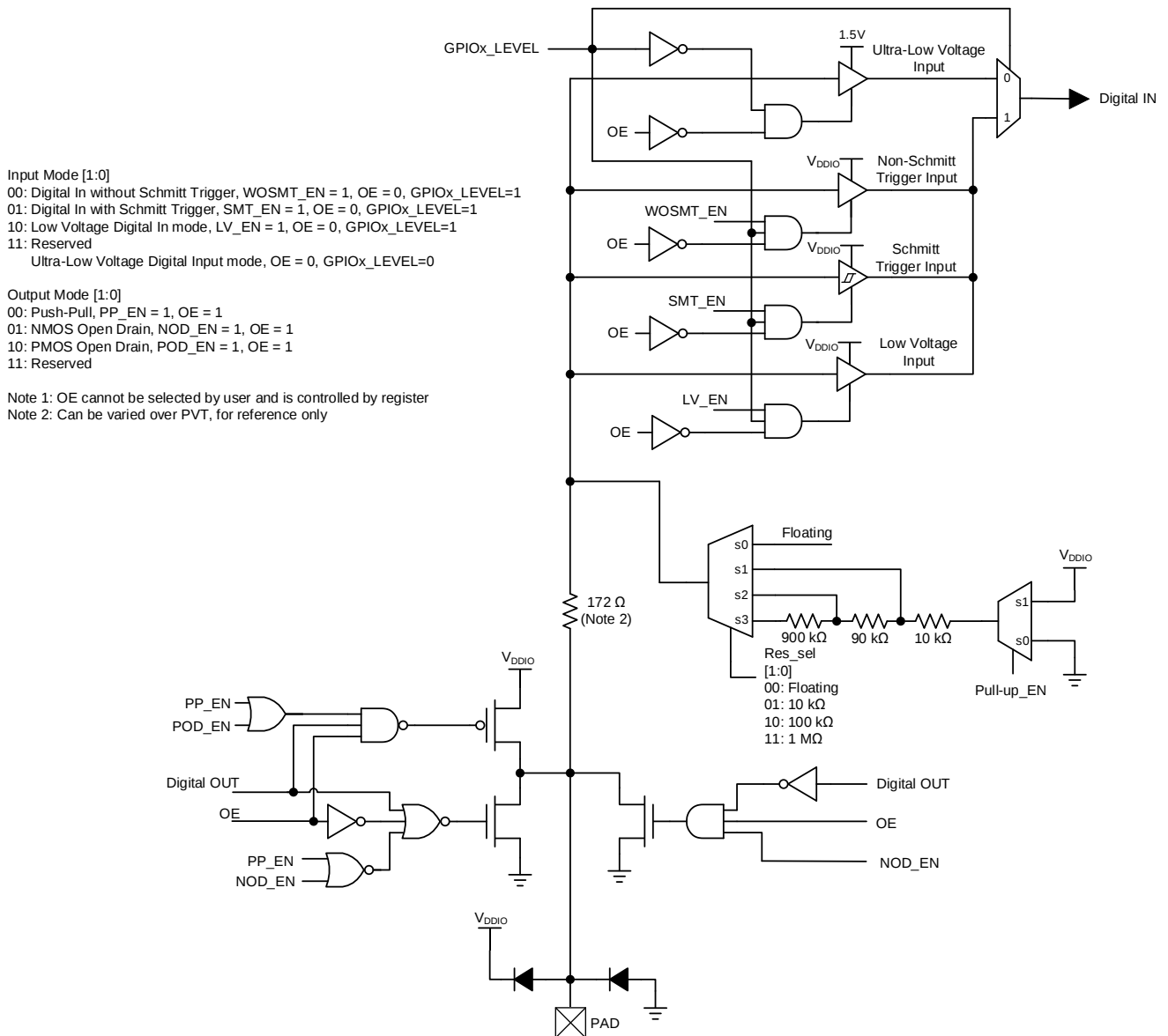
Figure 16. High Voltage GPIOs Structure
