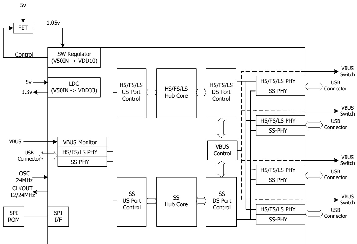
Figure 1-1. \mu PD720210 Block Diagram
