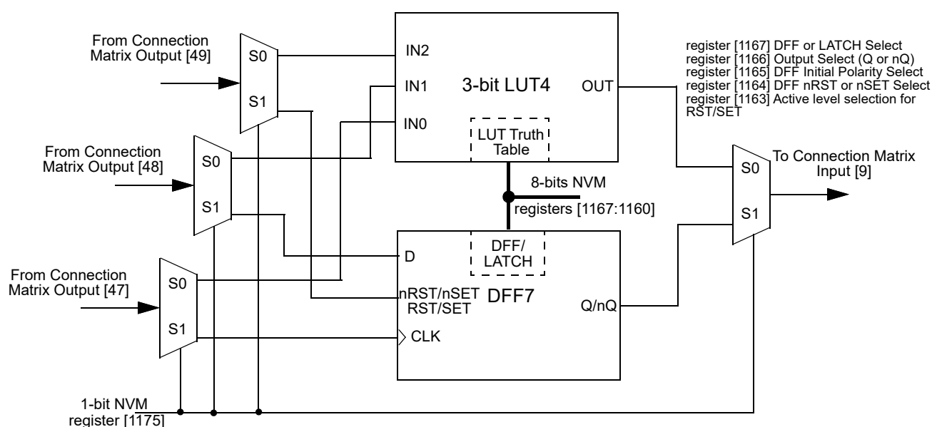
Figure 62. 3-bit LUT4 or DFF7
