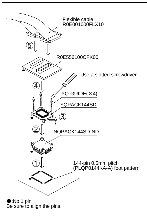
Figure 3 Connection procedure of the R0E556100CFK00
