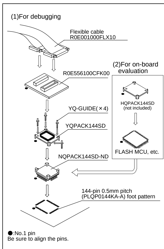
Figure 2 Usage of the R0E556100CFK00
