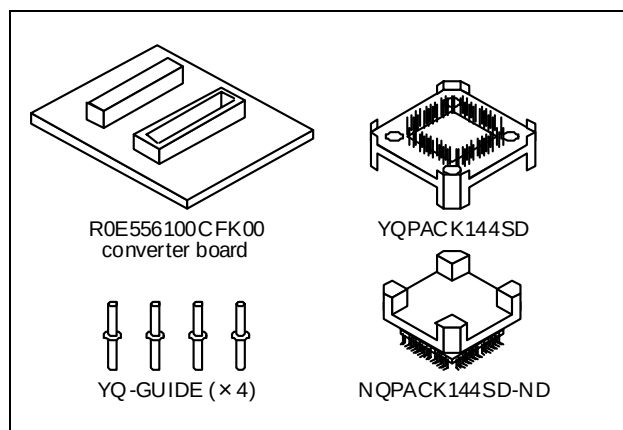
Figure 1 Package components of the R0E556100CFK00
