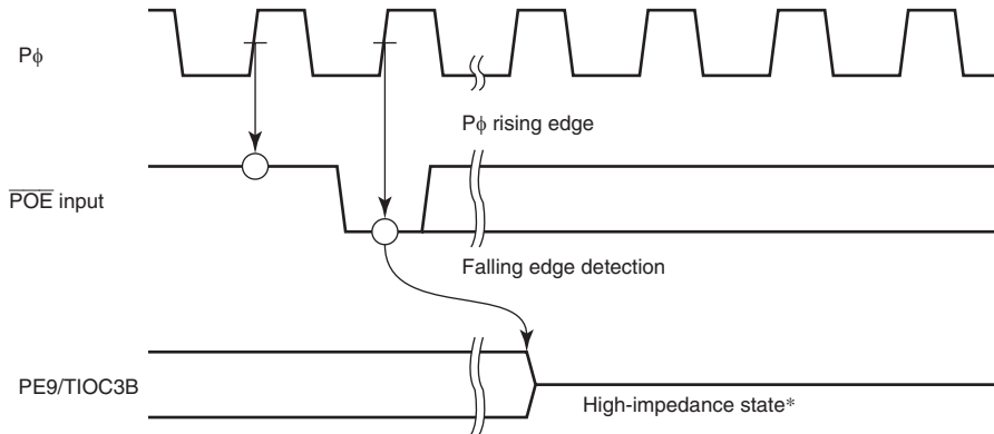
Figure 10.2 Falling Edge Detection
