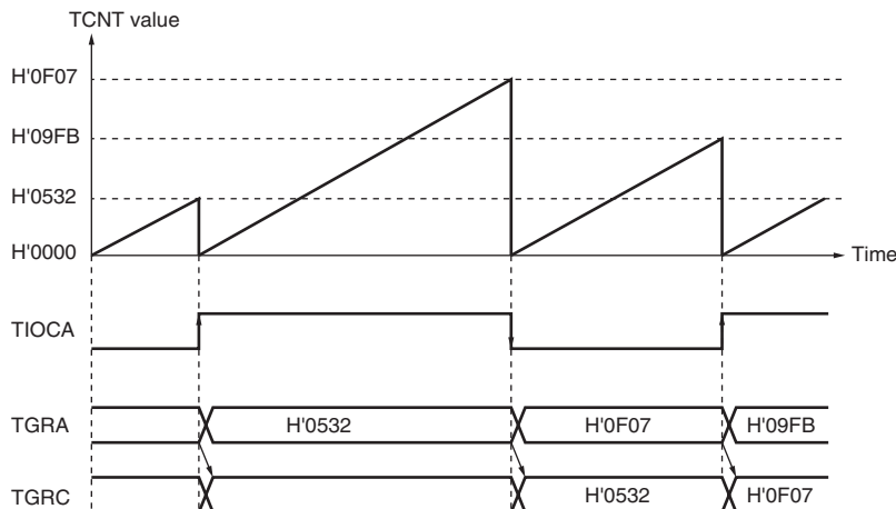
Figure 9.18 Example of Buffer Operation (2)
