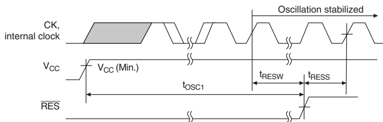
Figure 21.2 Power-On Oscillation Stabilization Time
