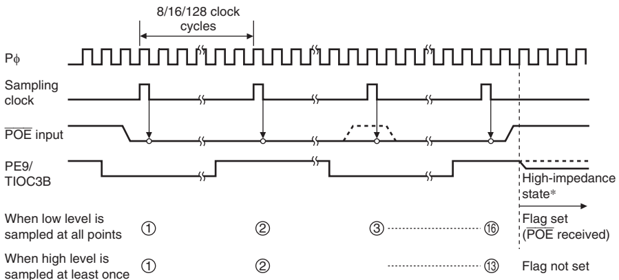
Figure 10.3 Low-Level Detection Operation
