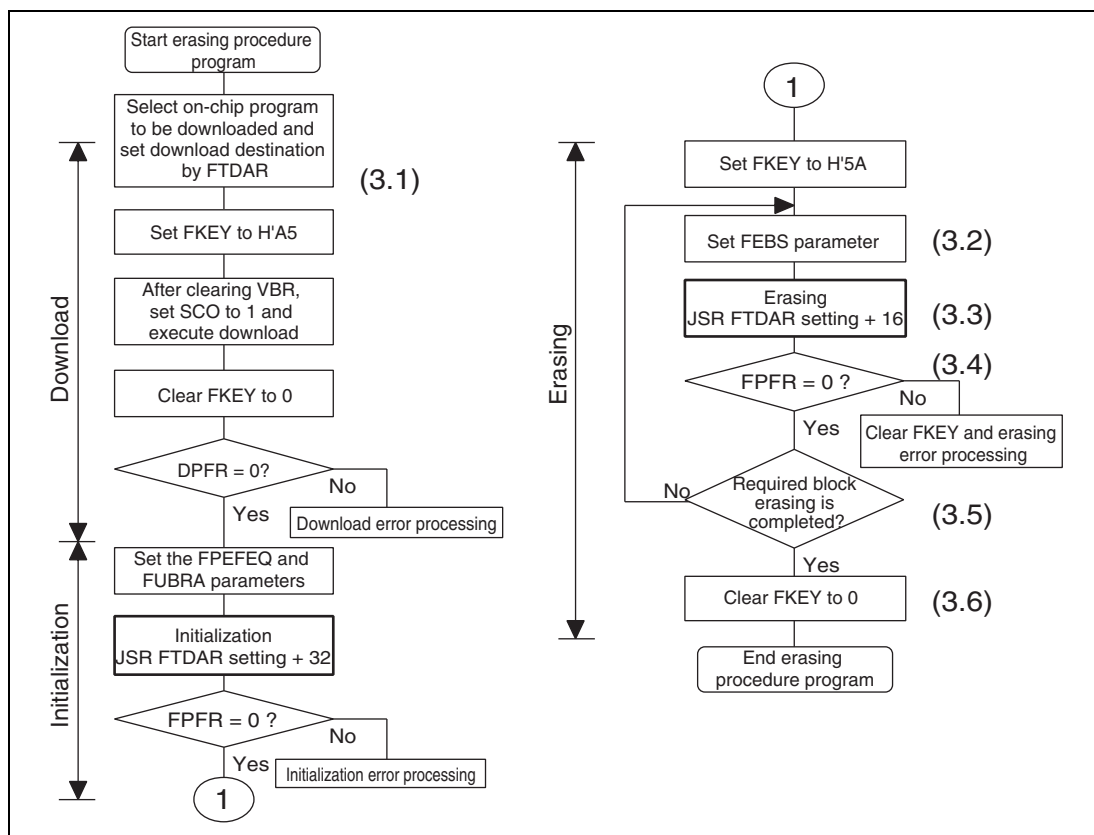
Figure 17.12 Erasing Procedure
