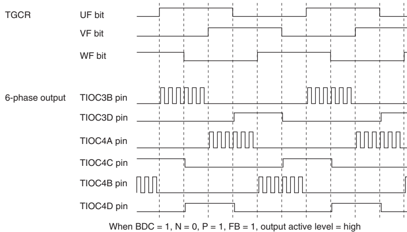
Figure 9.66 Example of Output Phase Switching by Means of UF, VF, WF Bit Settings (2)
