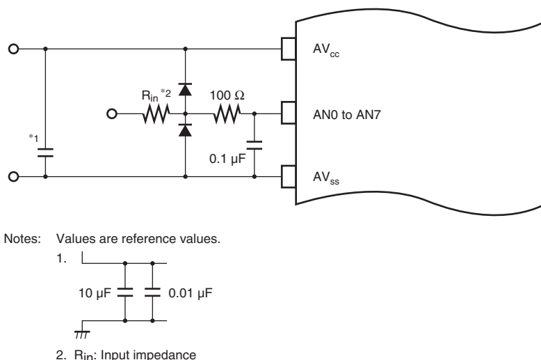
Figure 13.8 Example of Analog Input Protection Circuit
