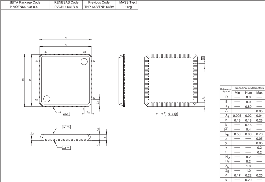
Figure C.4 VQFN-64
