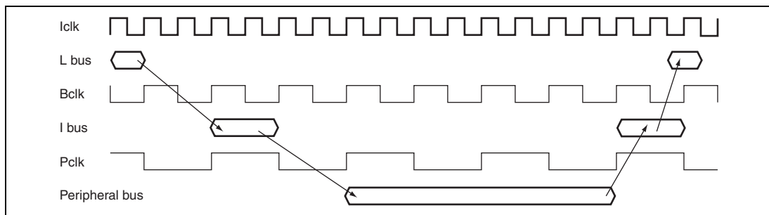
Figure 8.3 Timing of Read Access to the Peripheral Bus (Iclk:Bclk:Pclk = 4:2:1)
