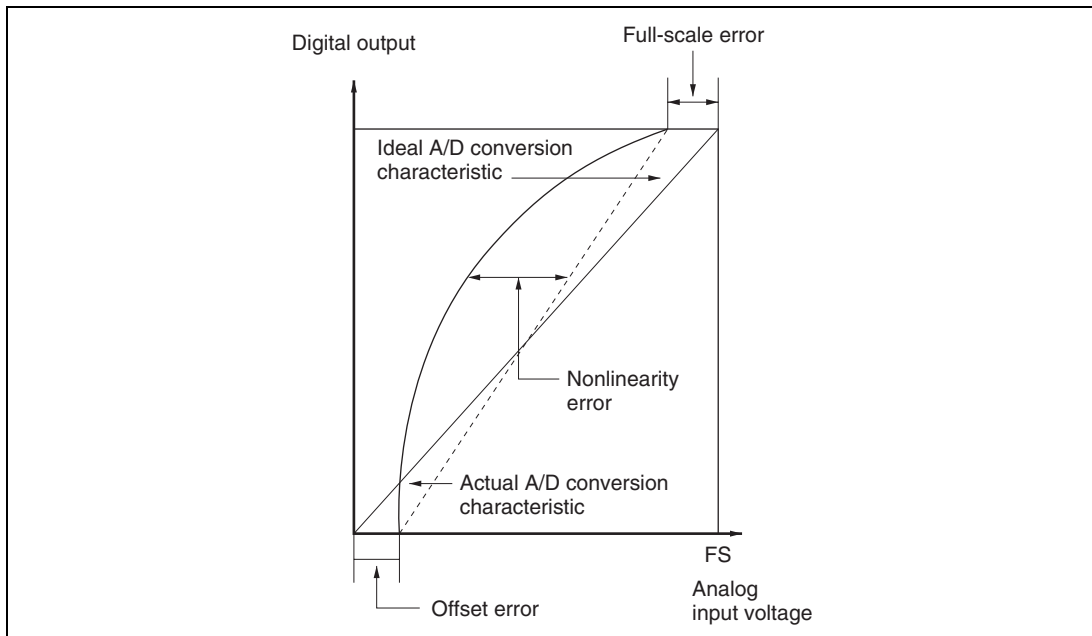
Figure 13.6 Definitions of A/D Conversion Accuracy
