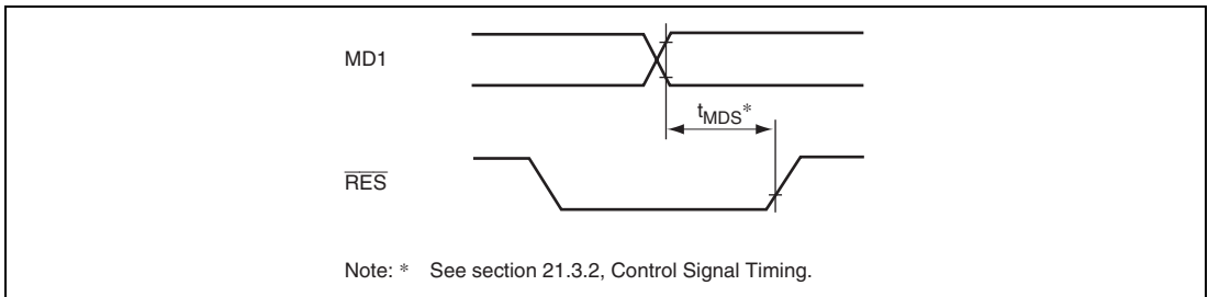
Figure 3.5 Reset Input Timing when Changing Operating Mode
