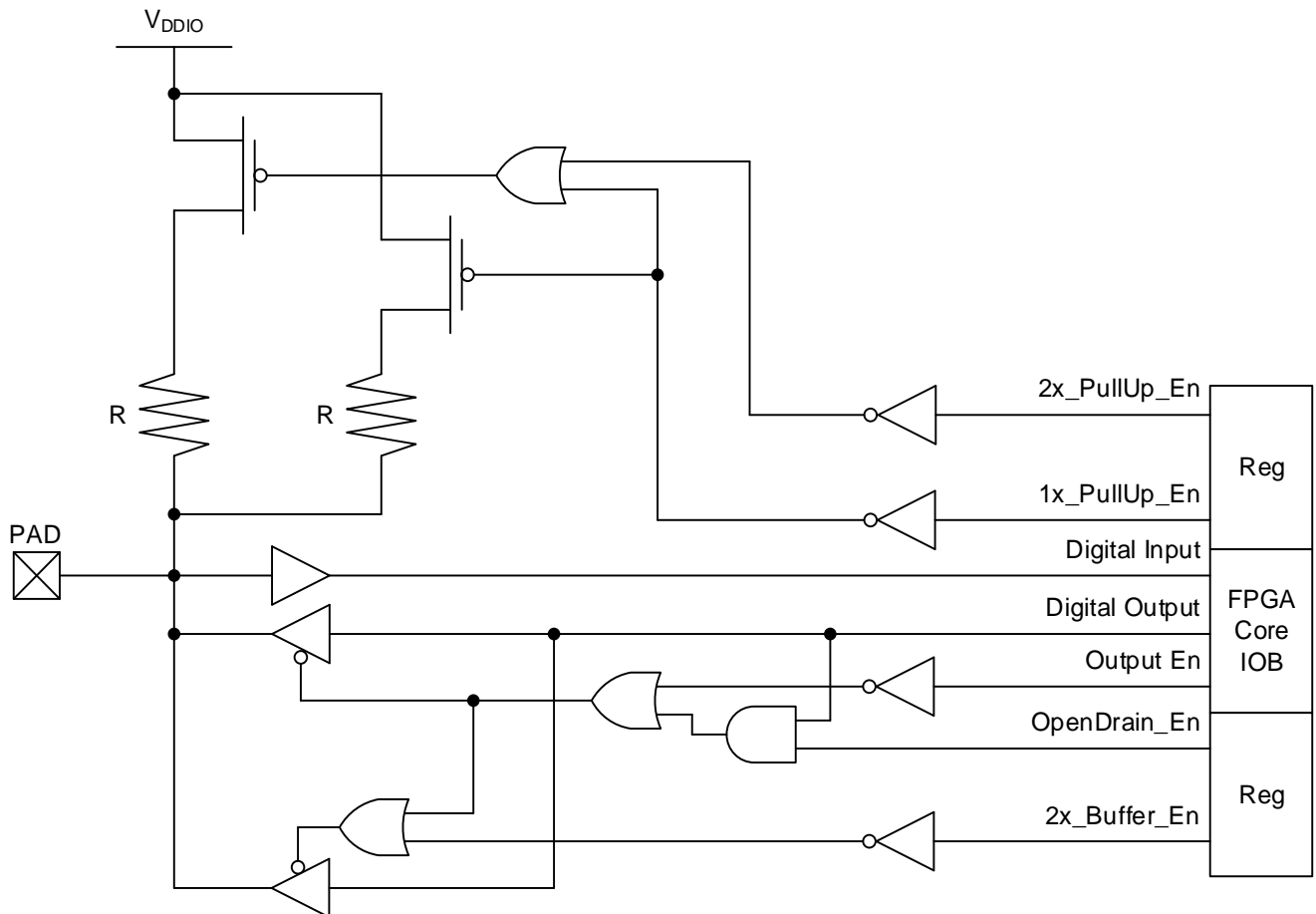
Figure 3. GPIO Buffers
