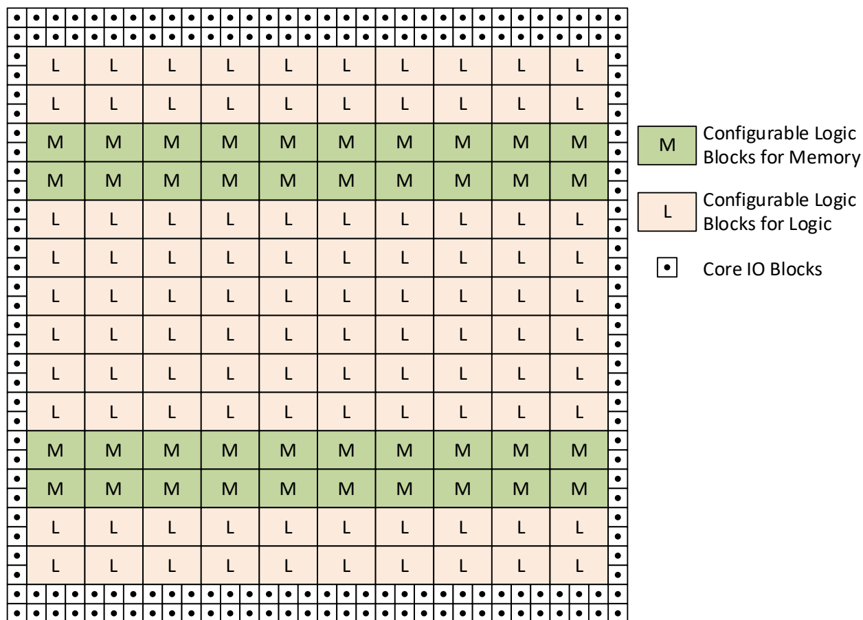
Figure 4. FPGA Core
