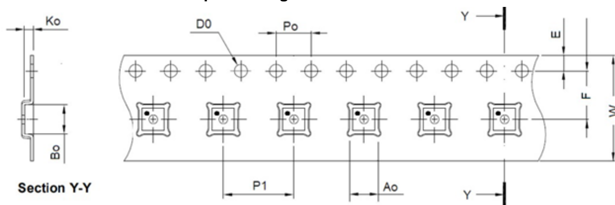
Figure 26. Carrier Tape Drawing for STQFN-24L
