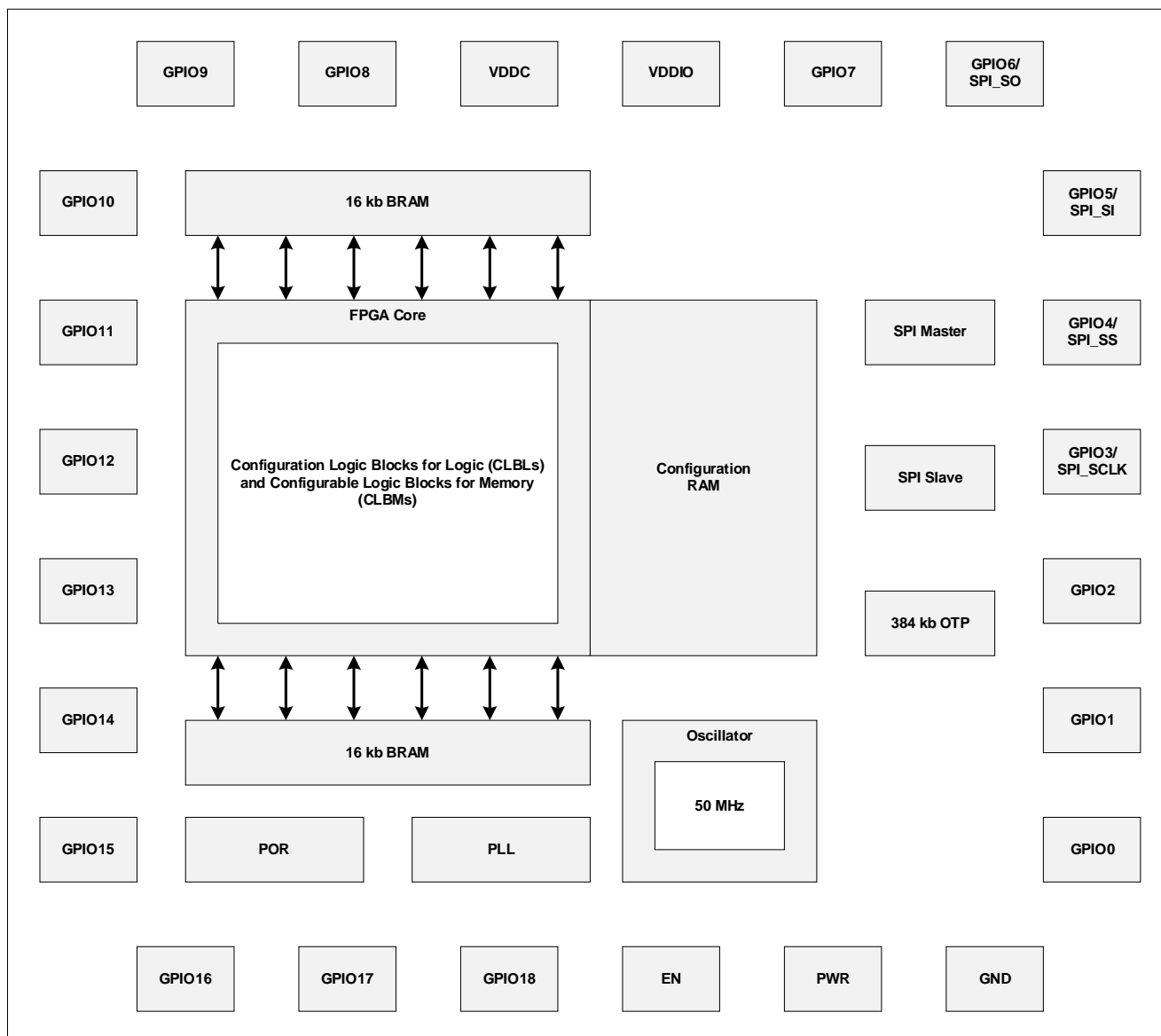
Figure 1. Block Diagram
