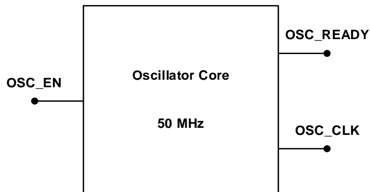
Figure 12. On-chip Oscillator
