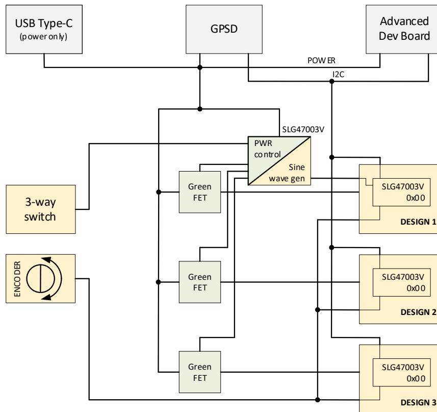
Figure 3. SLG47003V Demo Board Block Diagram
