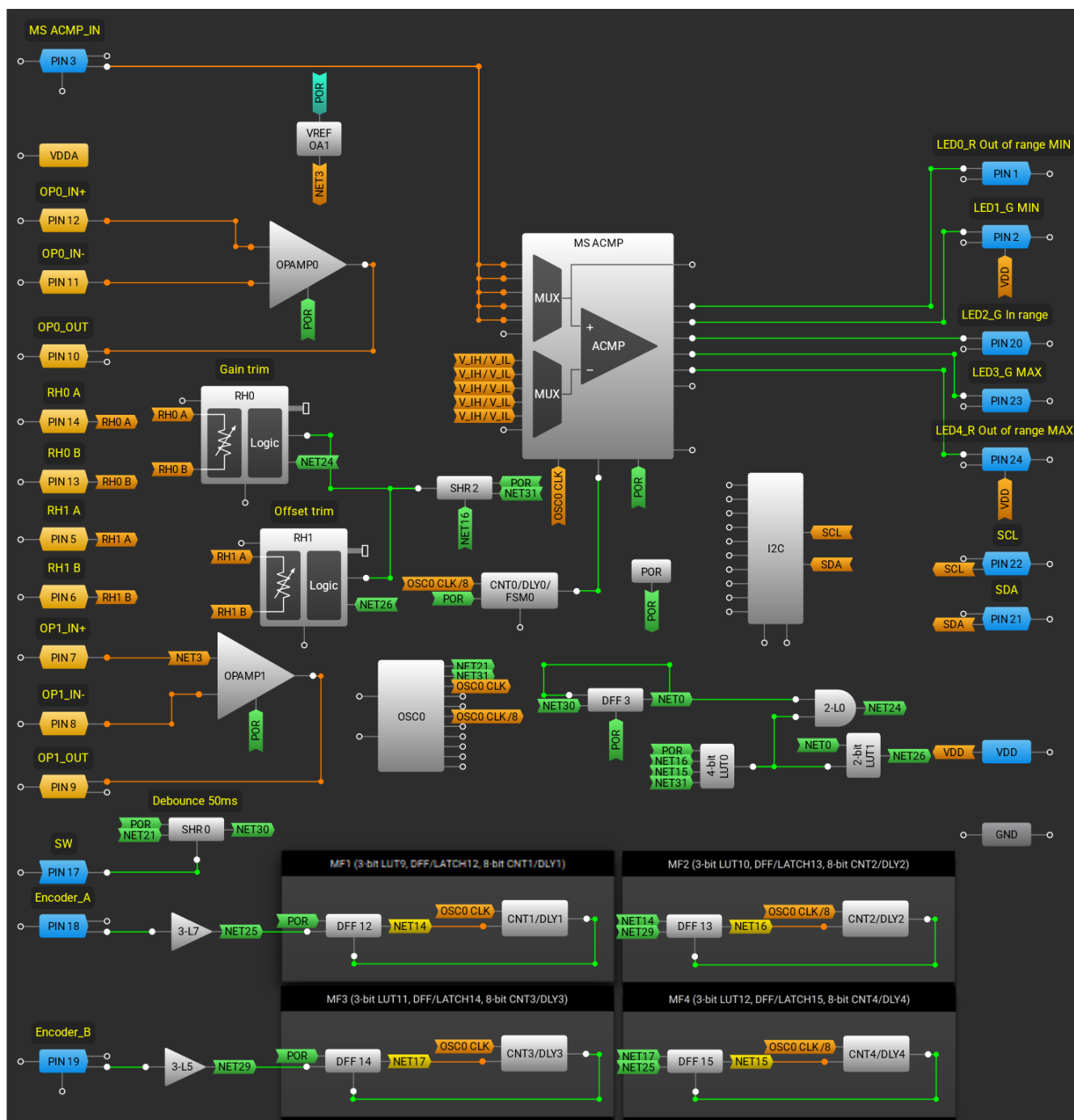
Figure 4. Go Configure Schematic of Offset and Gain Tuning
