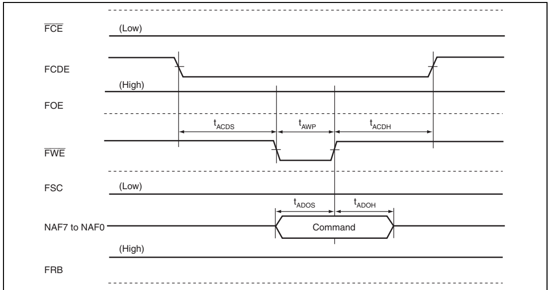
Figure 31.64 AND Type Flash Memory Command Issuance Timing
