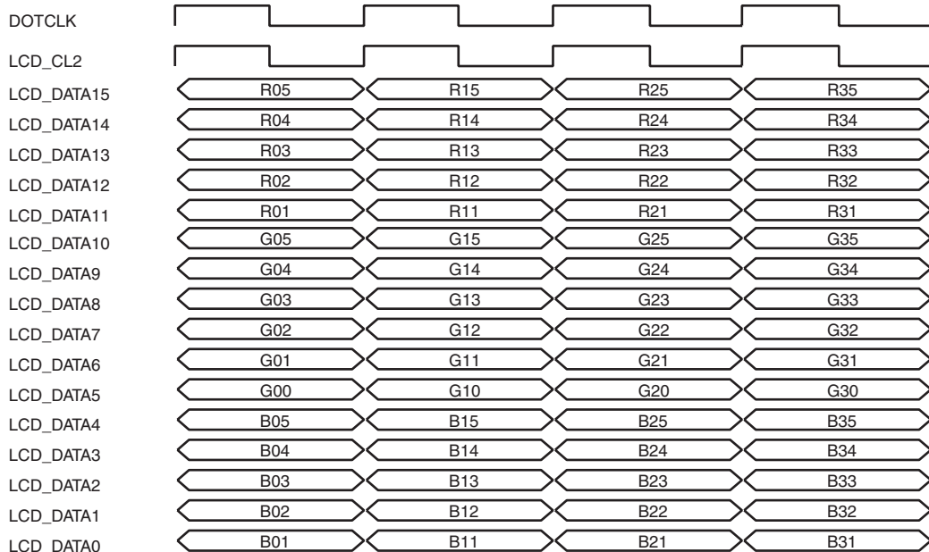
Figure 24.22 Clock and LCD Data Signal Example (TFT Color 16-Bit Data Bus Module)
