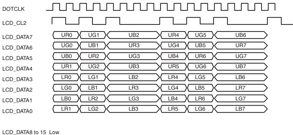
Figure 24.19 Clock and LCD Data Signal Example (DSTN Color 8-Bit Data Bus Module)
