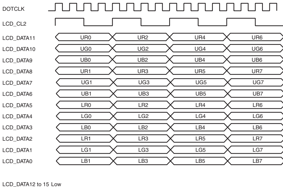
Figure 24.20 Clock and LCD Data Signal Example (DSTN Color 12-Bit Data Bus Module)
