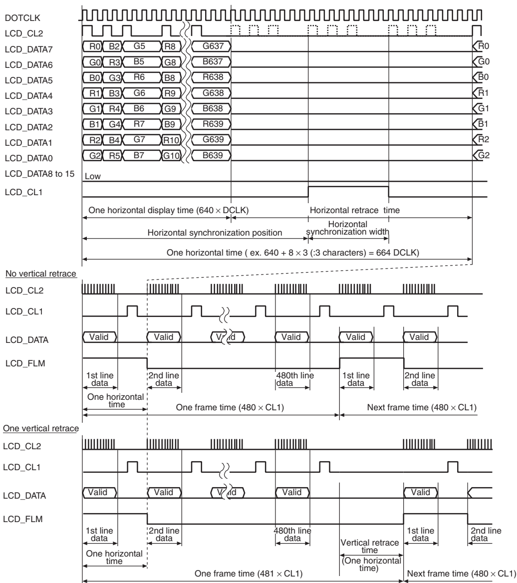
Figure 24.23 Clock and LCD Data Signal Example (8-Bit Interface Color 640 × 480)
