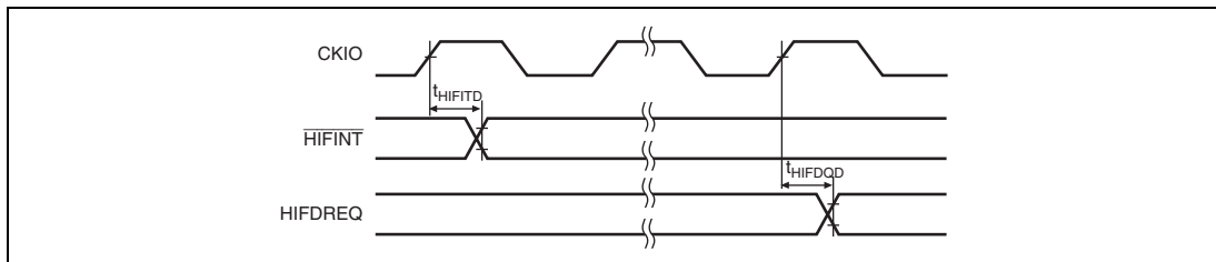
Figure 29.56 \overline{\text{HIFINT}} /HIFDREQ Timing
