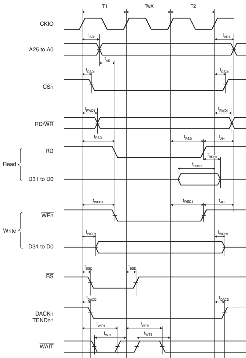
Figure 29.12 Basic Bus Timing for Normal Space (One External Wait Cycle)
