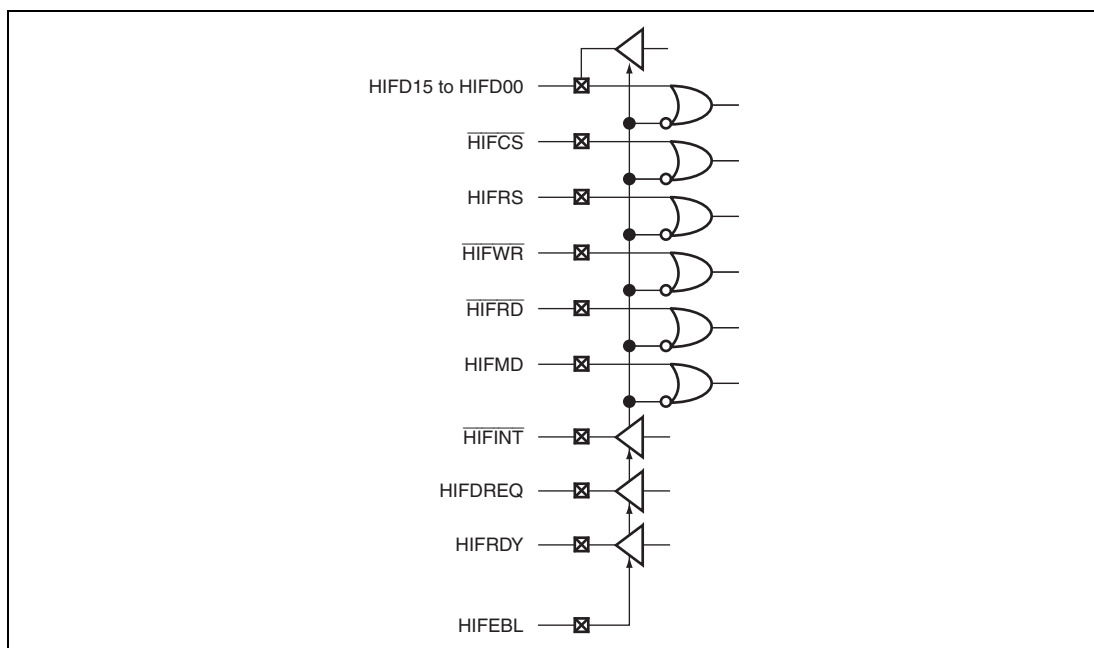
Figure 20.11 Image of High-Impedance Control of HIF Pins by HIFEBL Pin
