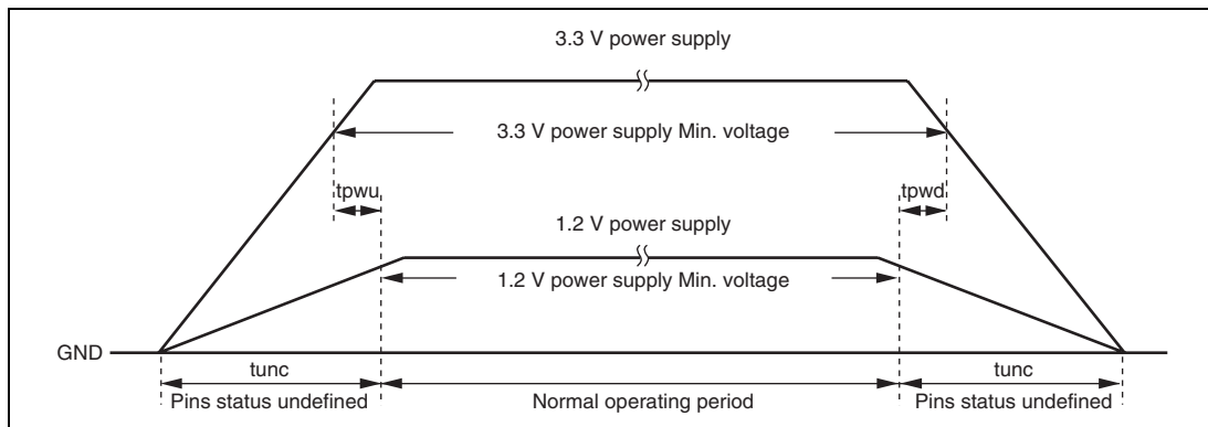
Figure 29.1 Power-on/Power-off Sequence
