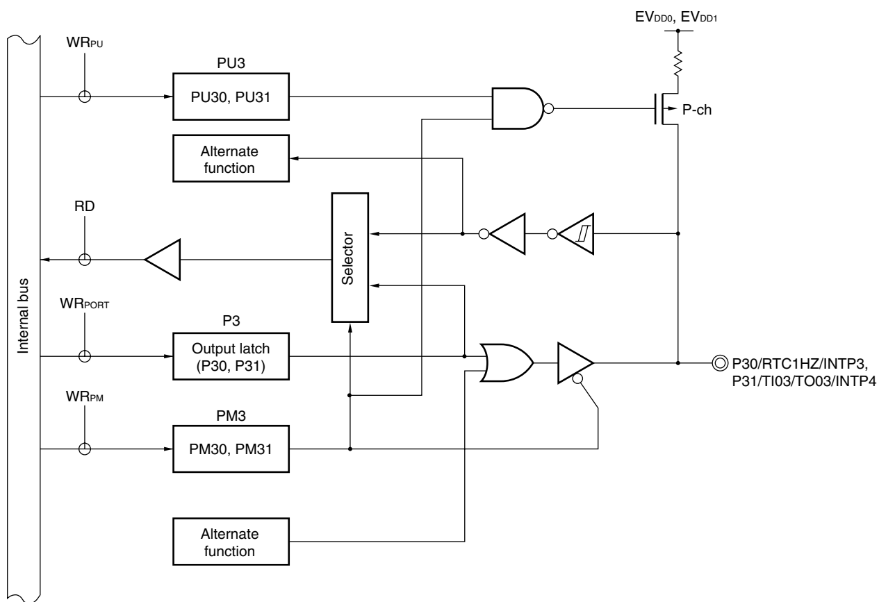
Figure 6-14. Block Diagram of P30 and P31
