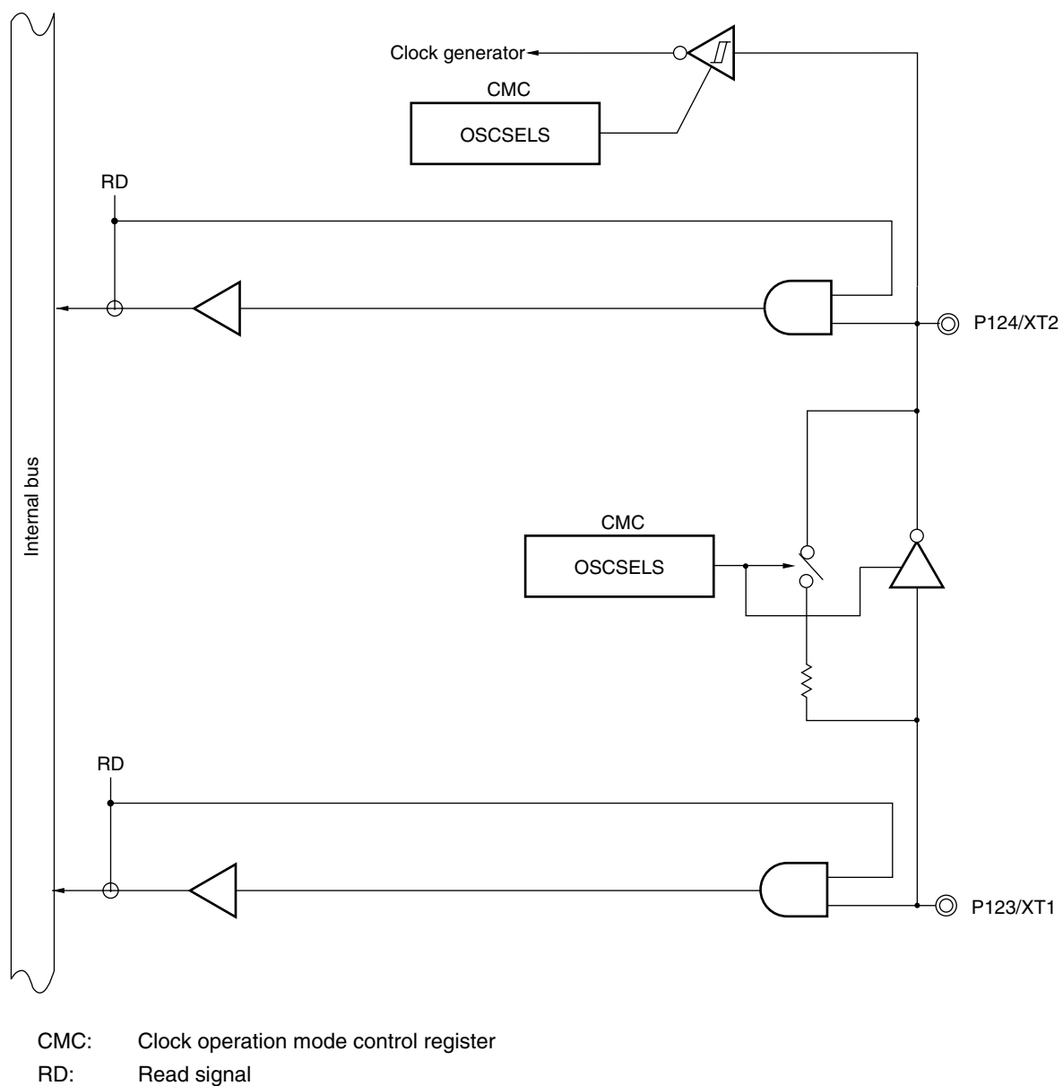
Figure 6-44. Block Diagram of P123 and P124
