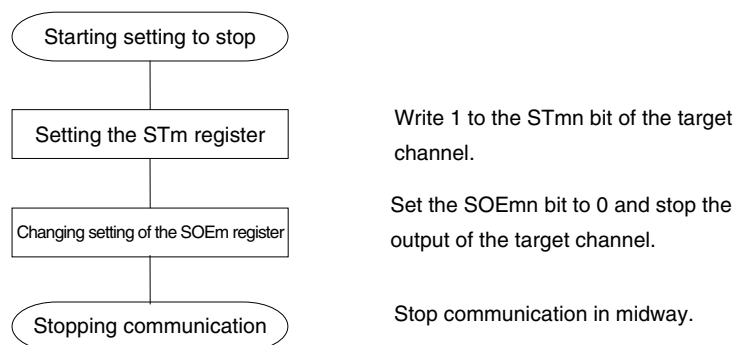
Figure 14-46. Procedure for Stopping Master Transmission/Reception
