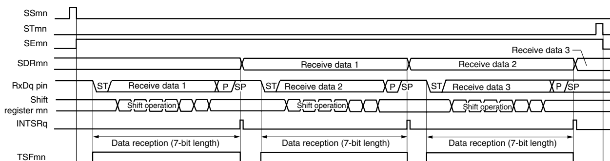
Figure 14-87. Timing Chart of UART Reception
