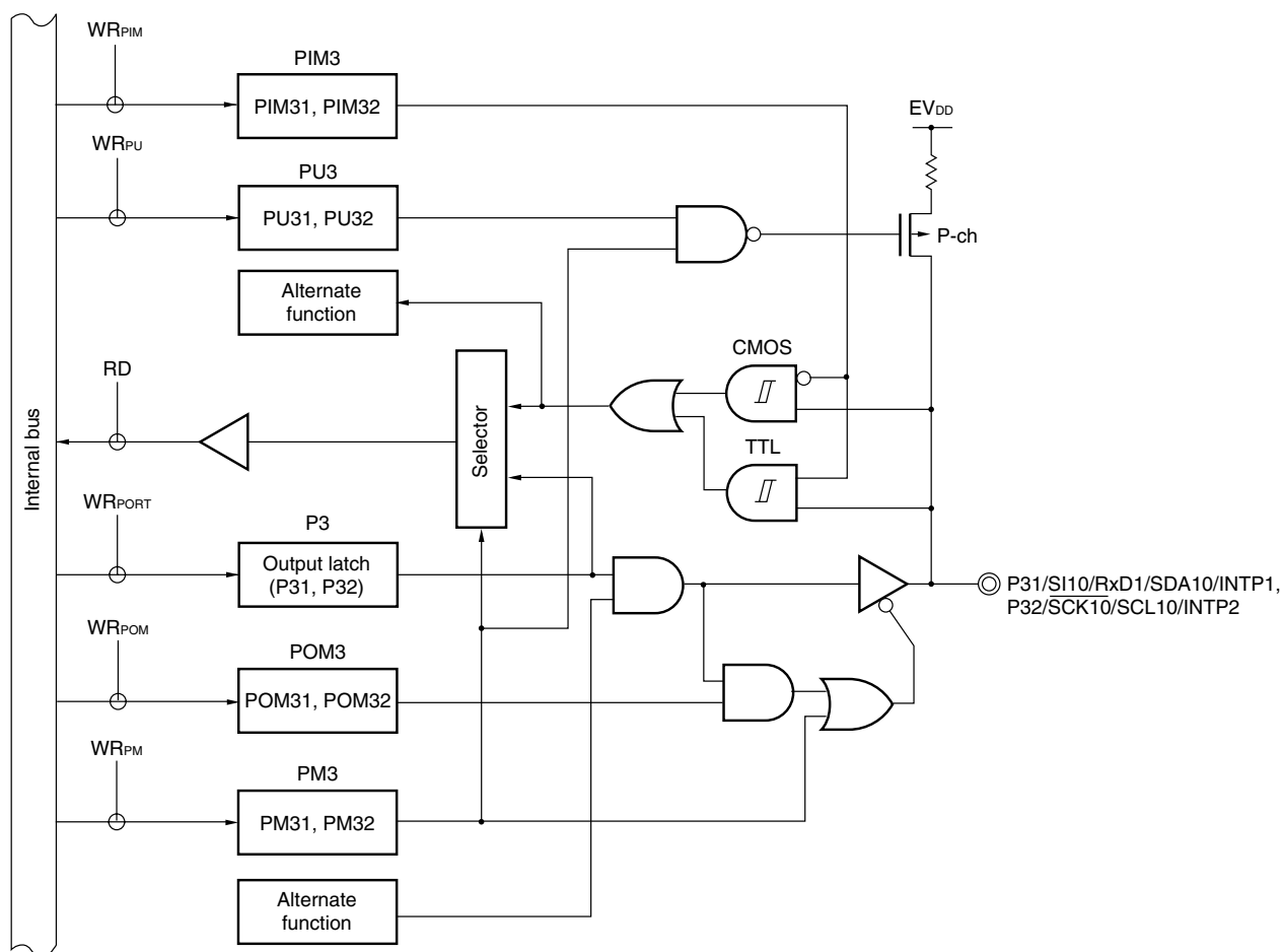
Figure 5-7. Block Diagram of P31 and P32
