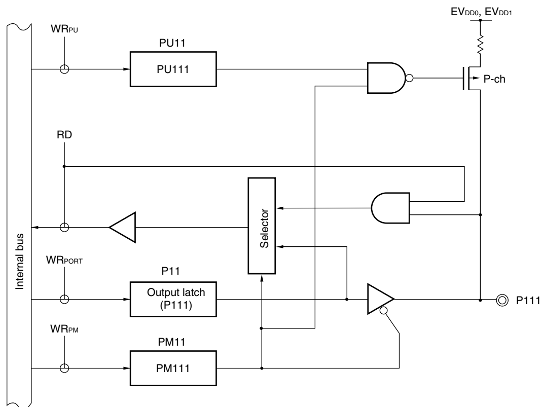
Figure 6-41. Block Diagram of P11
