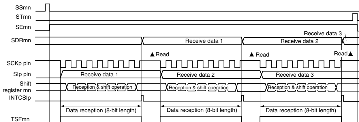
Figure 14-64. Timing Chart of Slave Reception (in Single-Reception Mode)
