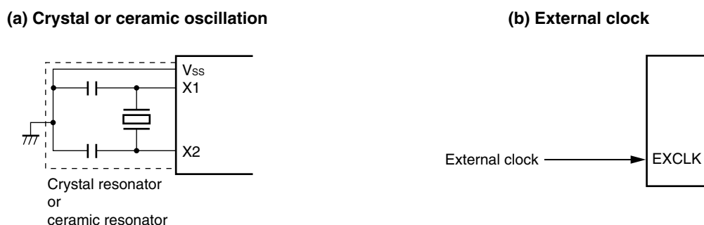
Figure 7-13. Example of External Circuit of X1 Oscillator
