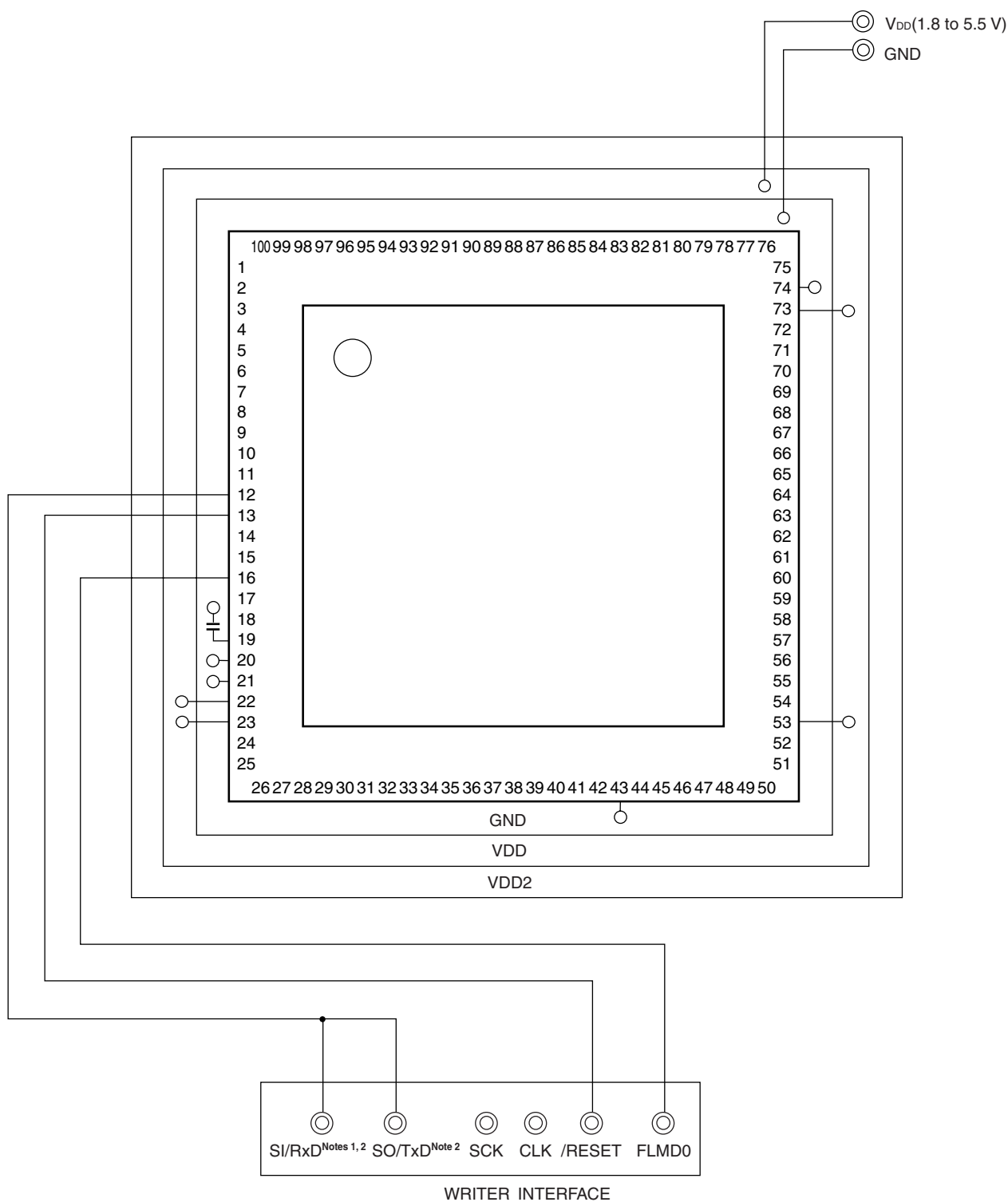
Figure 26-8. Example of Wiring Adapter for Flash Memory Writing (78K0R/KG3-L, LQFP (14x14))
