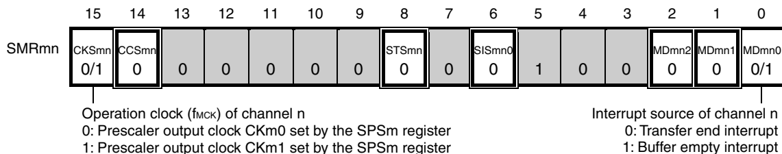
Figure 14-36. Example of Contents of Registers for Master Reception of 3-Wire Serial I/O (CSI00, CSI01, CSI10, CSI20, CSI40, CSI41) (1/2)
