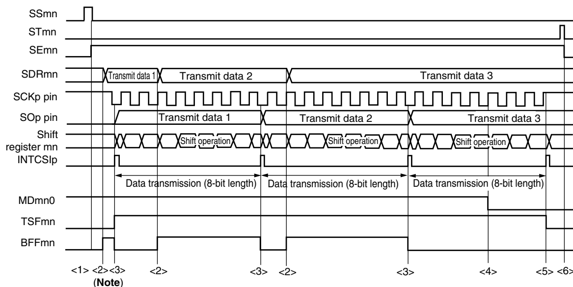
Figure 14-58. Timing Chart of Slave Transmission (in Continuous Transmission Mode)
