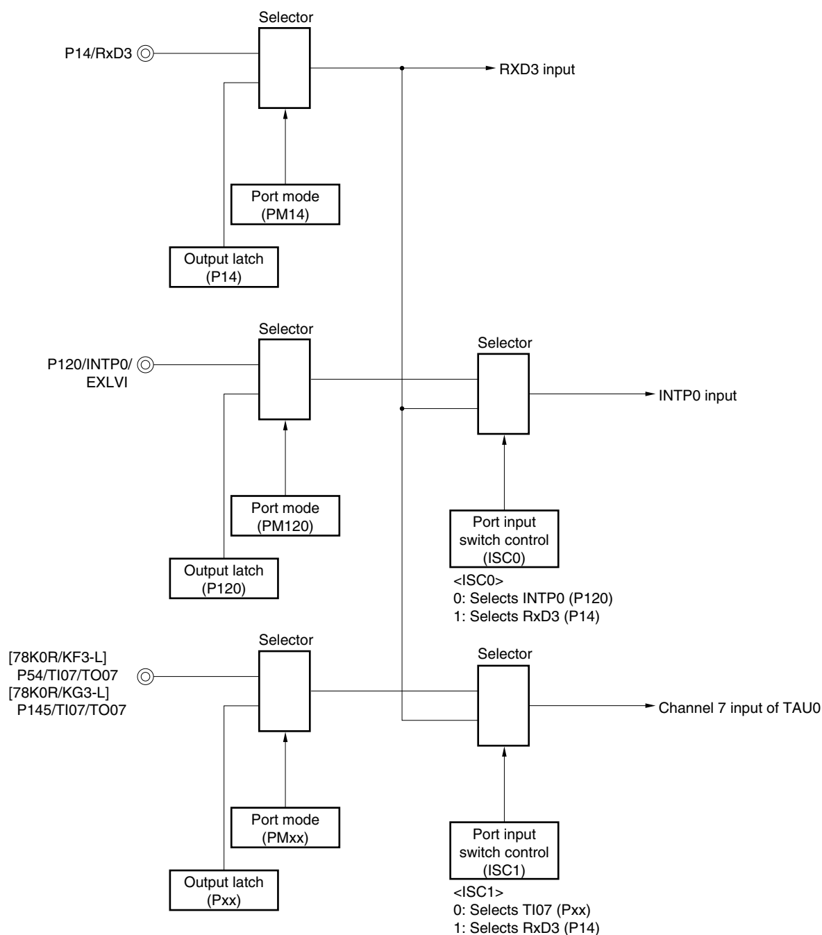
Figure 14-96 Port Configuration for Manipulating Reception of LIN (78K0R/KF3-L, 78K0R/KG3-L)
