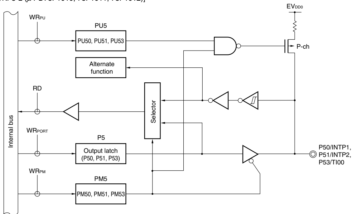
Figure 6-23. Block Diagram of P50, P51, and P53
