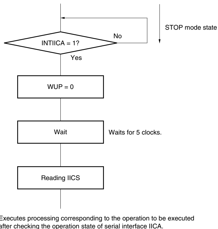
Figure 15-23. Flow When Setting WUP = 0 upon Address Match (Including Extension Code Reception)
