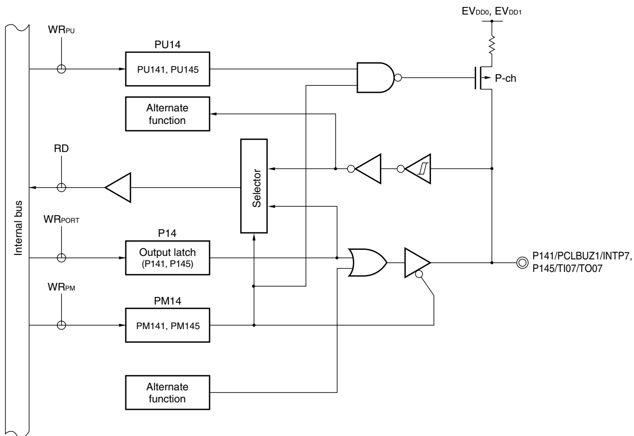
Figure 6-48. Block Diagram of P141 and P145
