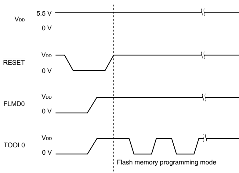
Figure 26-15. Flash Memory Programming Mode
