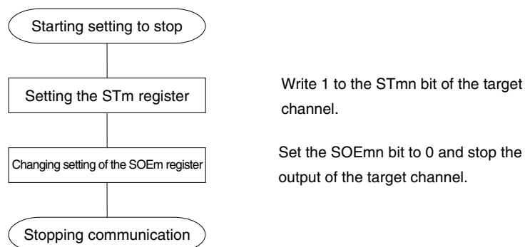
Figure 14-68. Procedure for Stopping Slave Transmission/Reception
