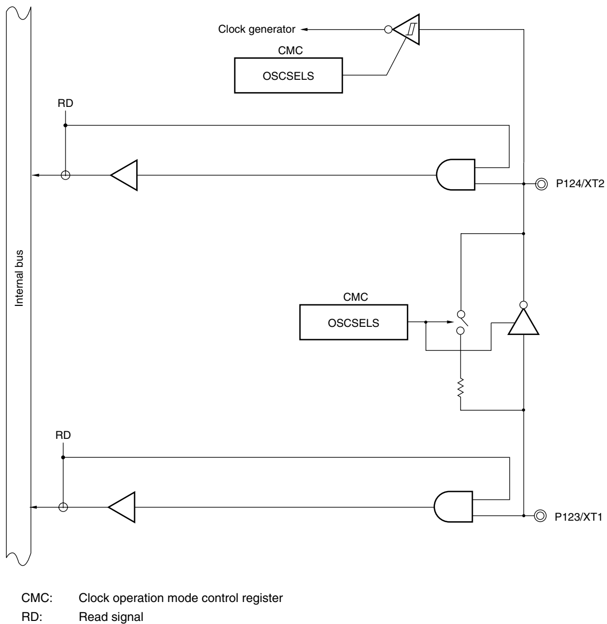
Figure 5-24. Block Diagram of P123 and P124
