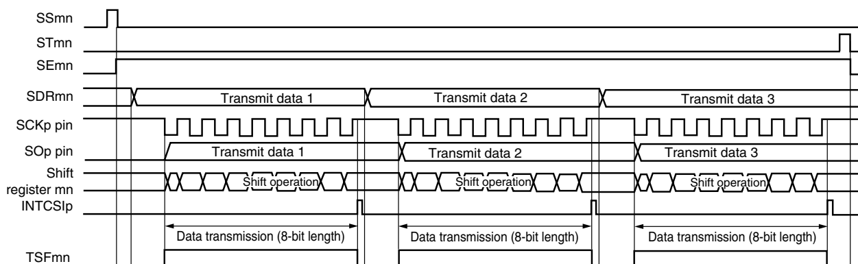
Figure 14-56. Timing Chart of Slave Transmission (in Single-Transmission Mode)
