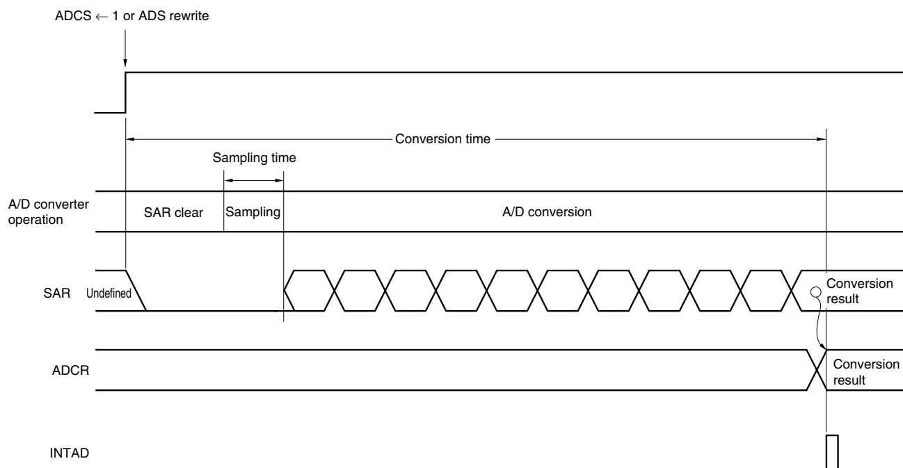
Figure 13-12. Basic Operation of A/D Converter
