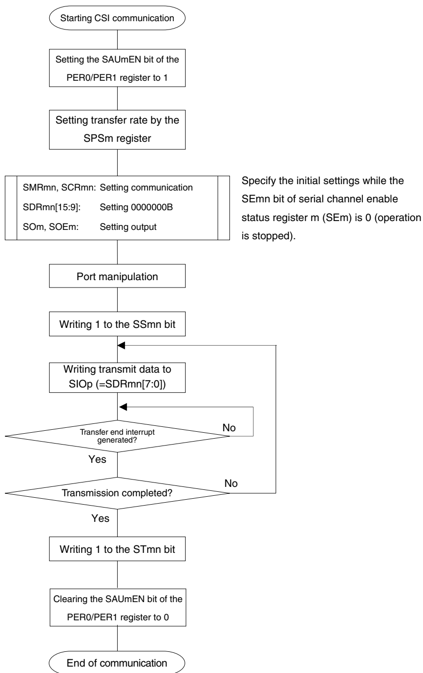
Figure 14-57. Flowchart of Slave Transmission (in Single-Transmission Mode)
