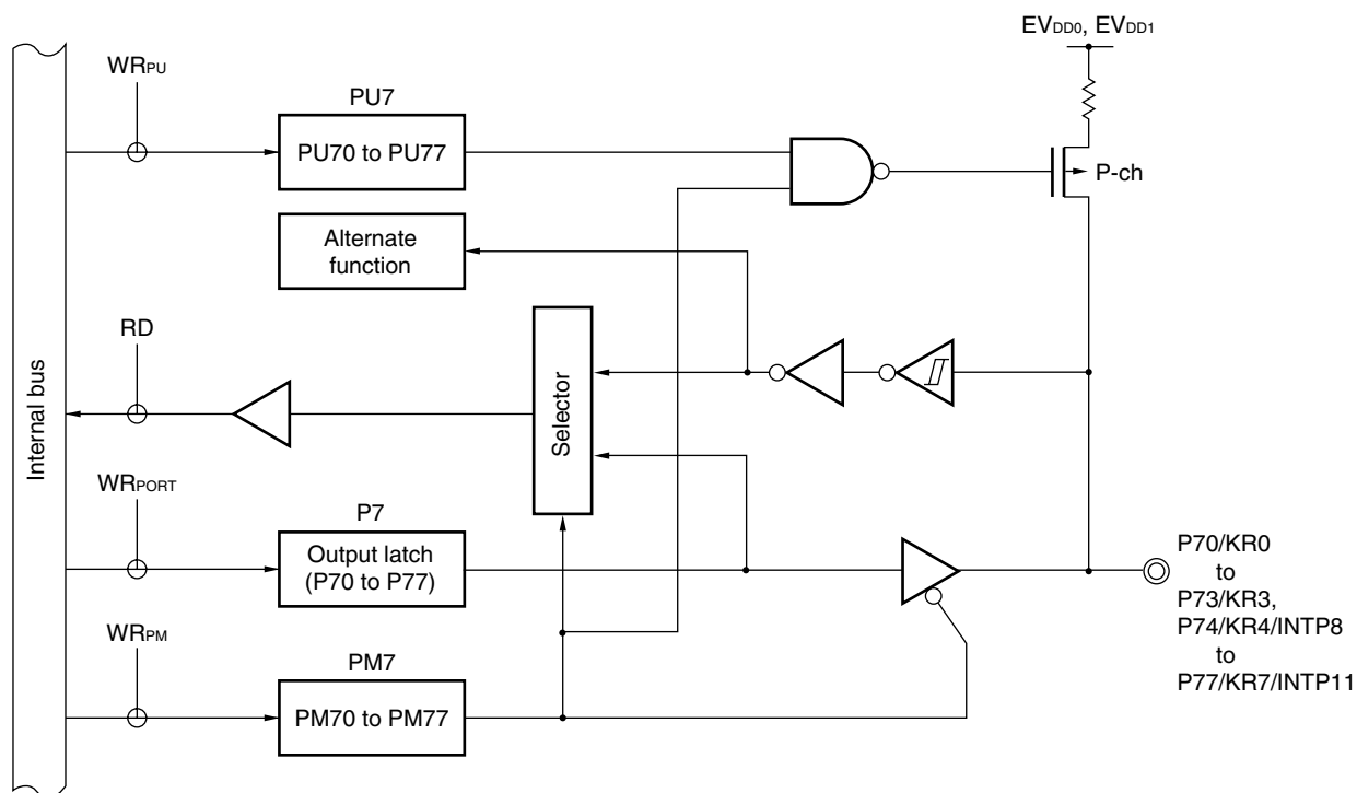
Figure 6-37. Block Diagram of P70 to P77
