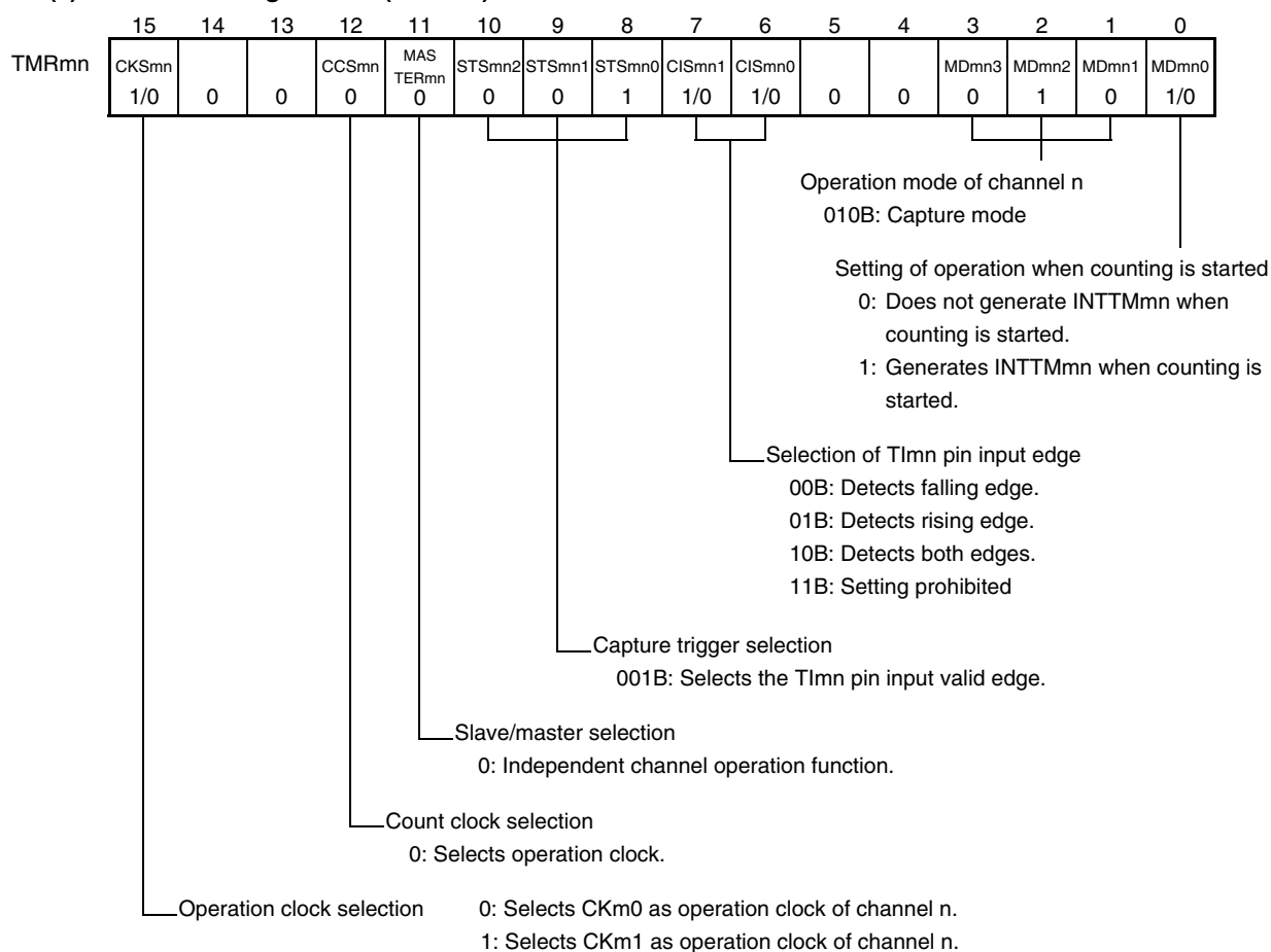
Figure 8-55. Example of Set Contents of Registers to Measure Input Pulse Interval
