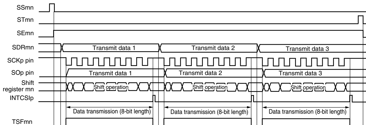
Figure 14-32. Timing Chart of Master Transmission (in Single-Transmission Mode) (Type 1: DAPmn = 0, CKPmn = 0)
