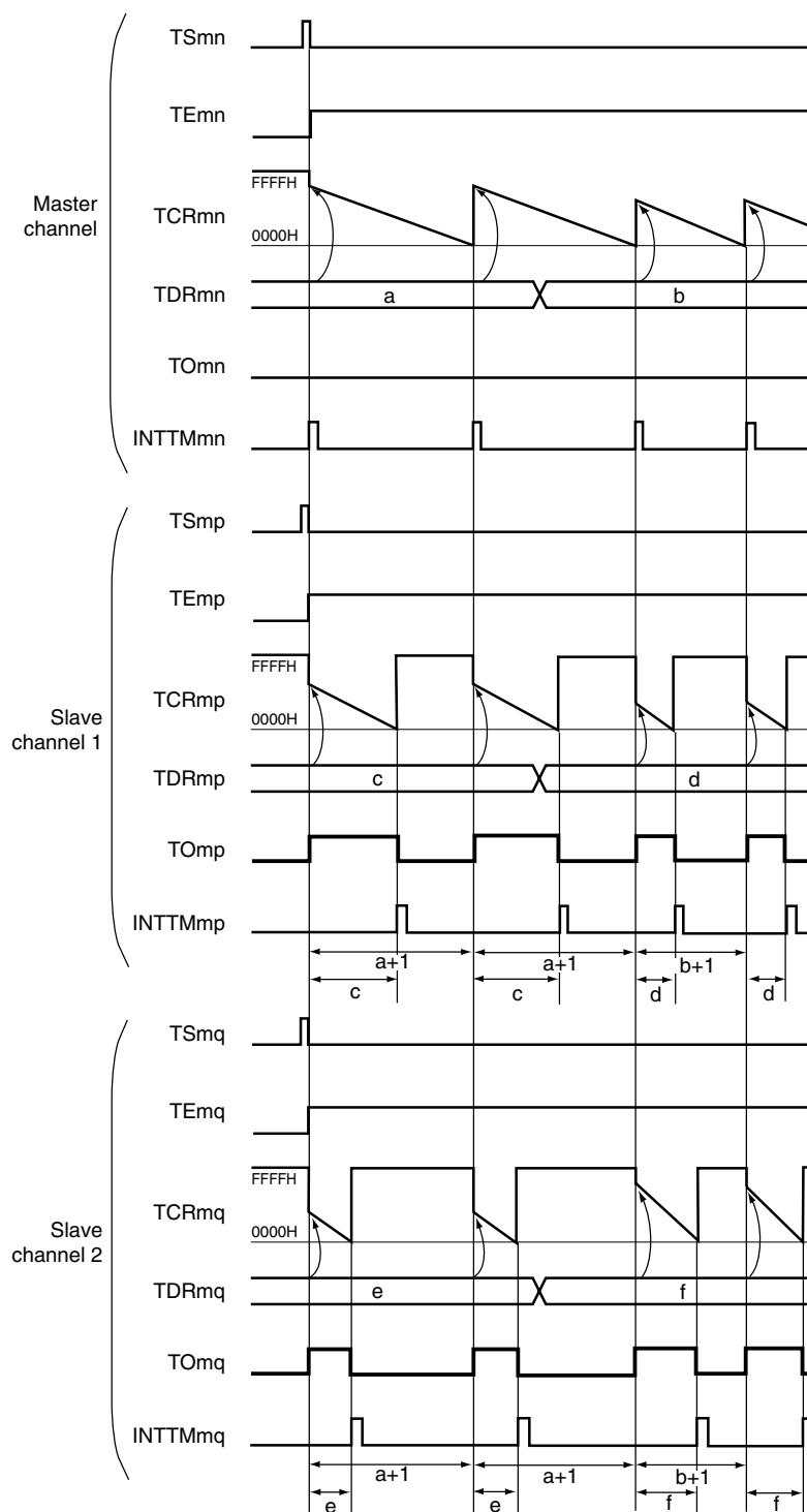
Figure 8-72. Example of Basic Timing of Operation as Multiple PWM Output Function (output two types of PWMs) (1/2)
