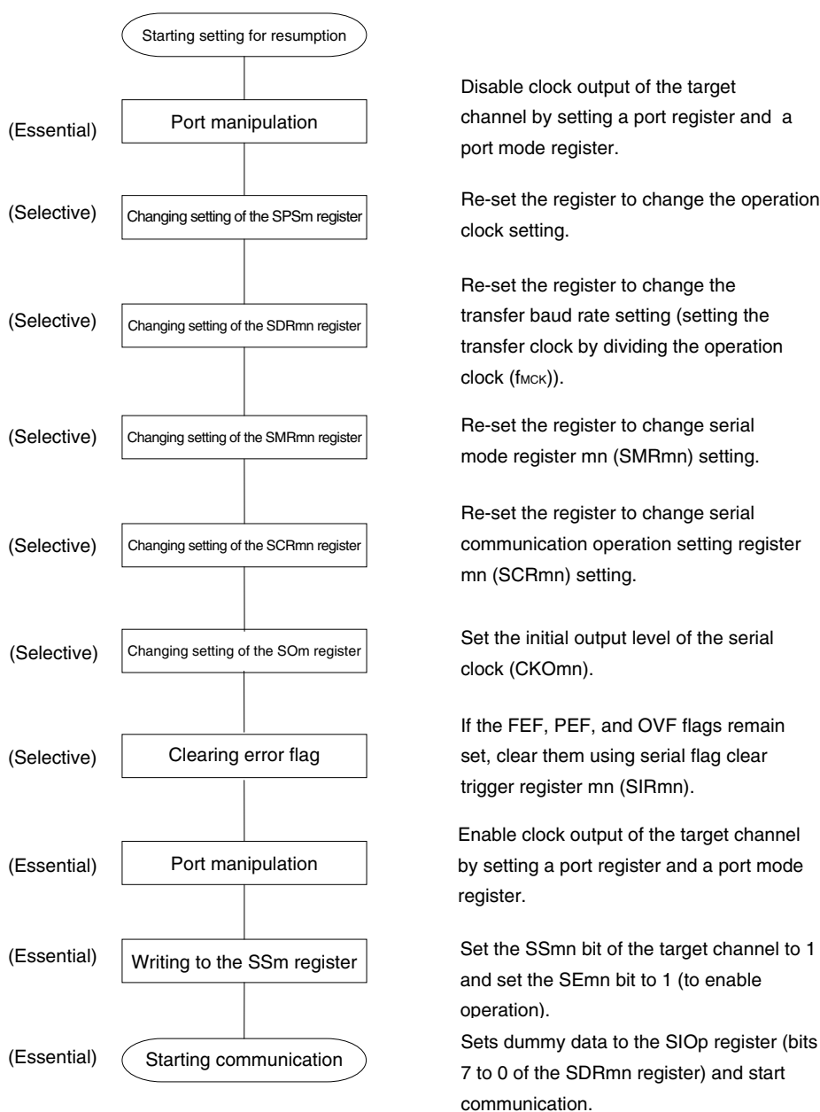
Figure 14-39. Procedure for Resuming Master Reception
