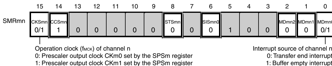
Figure 14-66. Example of Contents of Registers for Slave Transmission/Reception of 3-Wire Serial I/O (CSI00, CSI01, CSI10, CSI20, CSK40, CSK41) (1/2)
