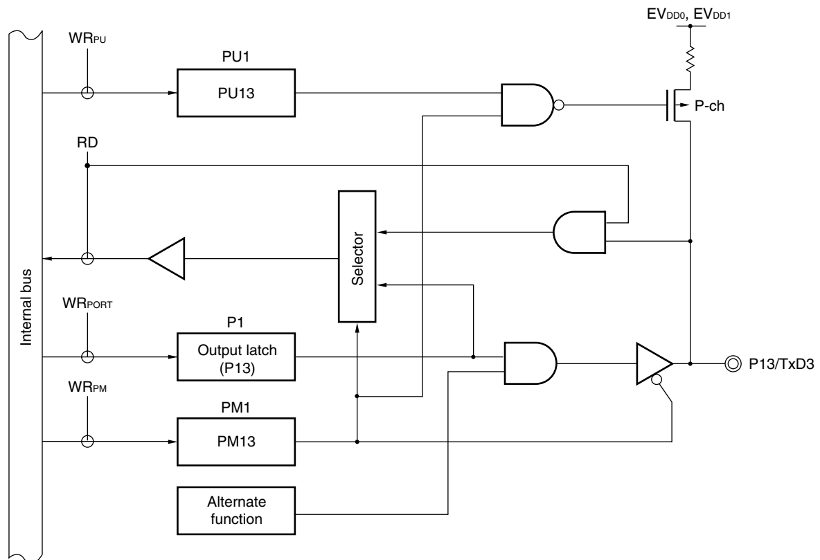
Figure 6-9. Block Diagram of P13
