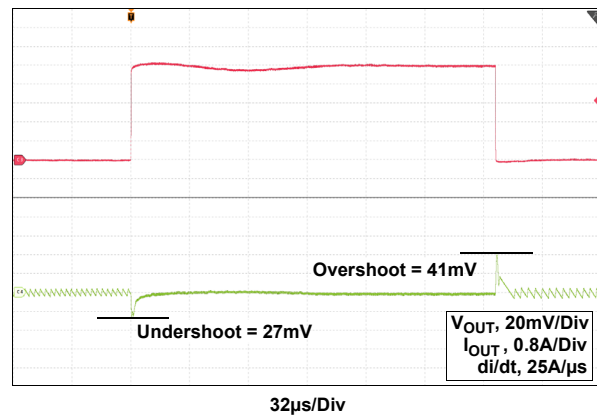
Load Step Slew Rate: 25A/µs, 0.1A to 4A 220nH Inductor (Cyttec PIFE25201T-R22MS) 2x22µF Capacitor (0603 6.3V Murata) 2x4.3µF Capacitor (0402 Low ESL Murata)
