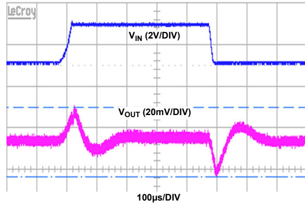
Figure 17. Single-Phase Line Transient, V_{OUT} = 1V , V_{IN} = 3.1V to 4.8V , Load = 4A, TR and TF = 15µs
