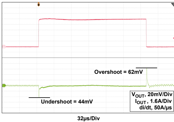
Load Step Slew Rate: 50A/µs, 0.1A to 8A 220nH Inductor (Cyttec PIFE25201T-R22MS) 4x22µF Capacitor (0603 6.3V Murata) 2x4.3µF Capacitor (0402 Low ESL Murata) 4x1µF Capacitor (0204 Taiyo Yuden)
