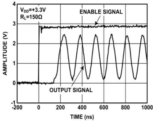
FIGURE 15. ENABLE TIME
