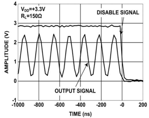
FIGURE 16. DISABLE TIME
