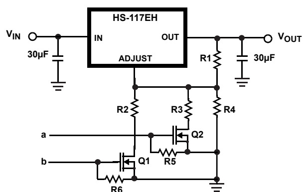
FIGURE 6. FOUR DIGITALLY PROGRAMMED OUTPUT VOLTAGES
