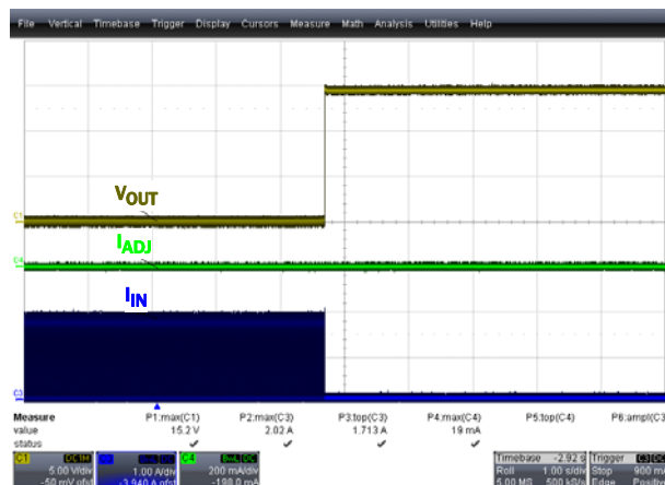
FIGURE 20. SHORT-CIRCUIT RECOVERY
