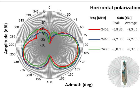
Figure 20. Radiation pattern for XZ-plane, horizontal polarization
