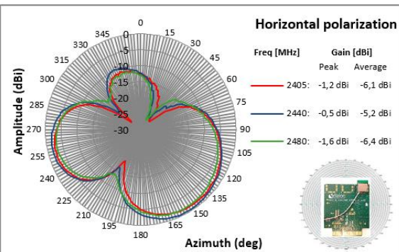
Figure 22. Radiation pattern for YZ-plane, horizontal polarization
